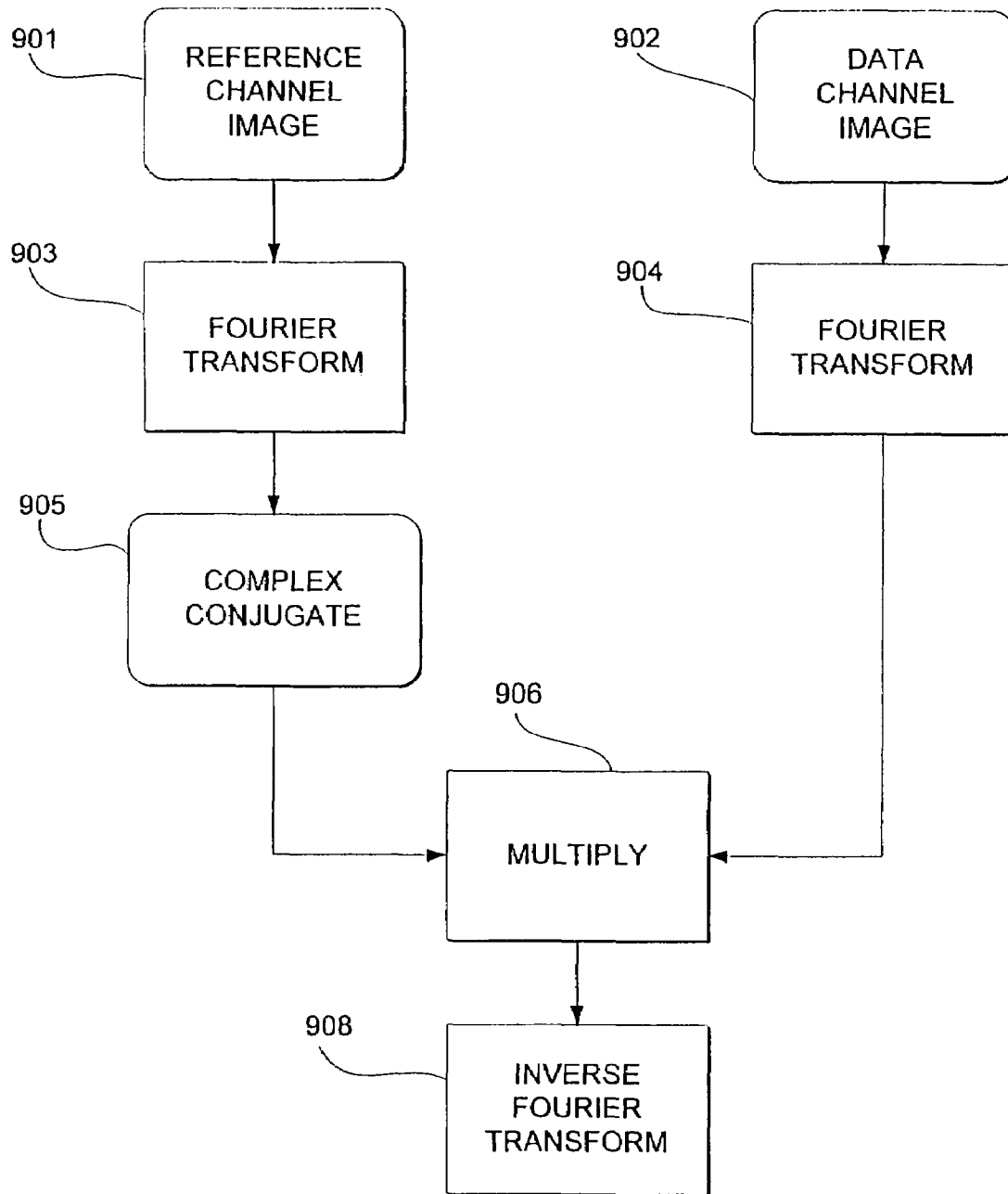
FIG. 9 CONVOLUTION AS MULTIPLICATION IN THE FREQUENCY DOMAIN
