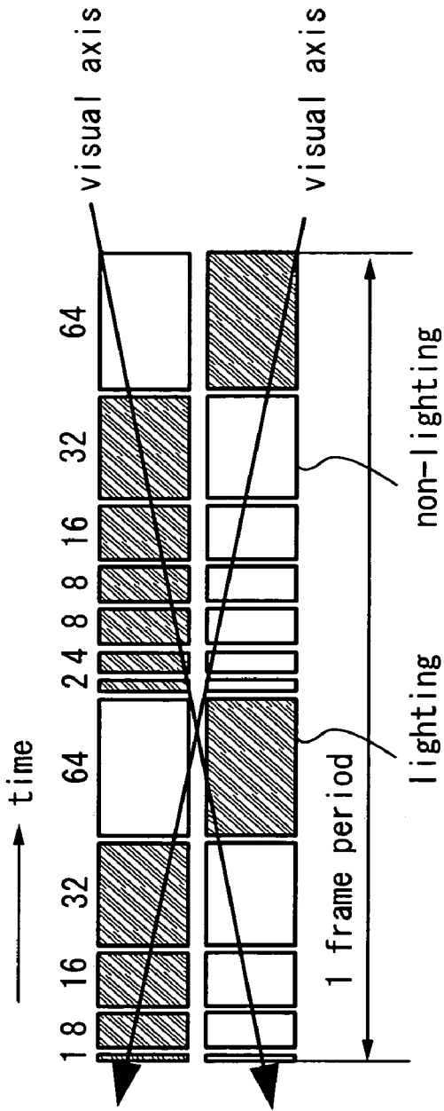
FIG. 50A pixel A gray scale level : 127 pixel B gray scale level : 128 PRIOR ART
