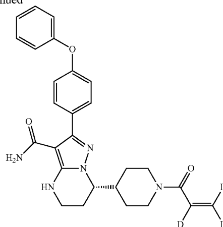
Deuterium-Labeled Compound 1
