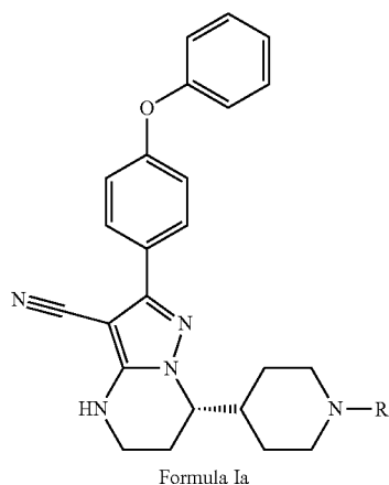
Formula Ia
