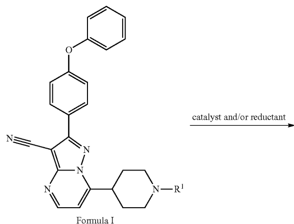
Formula I
