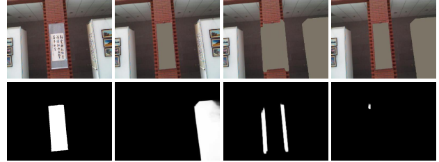
Figure 5. New label generation. The 1^{\text{st}} row: we iteratively hide the predicted salient region, where no region is hidden in the first image. The 2^{\text{nd}} row: the corresponding GT of the hidden image.
