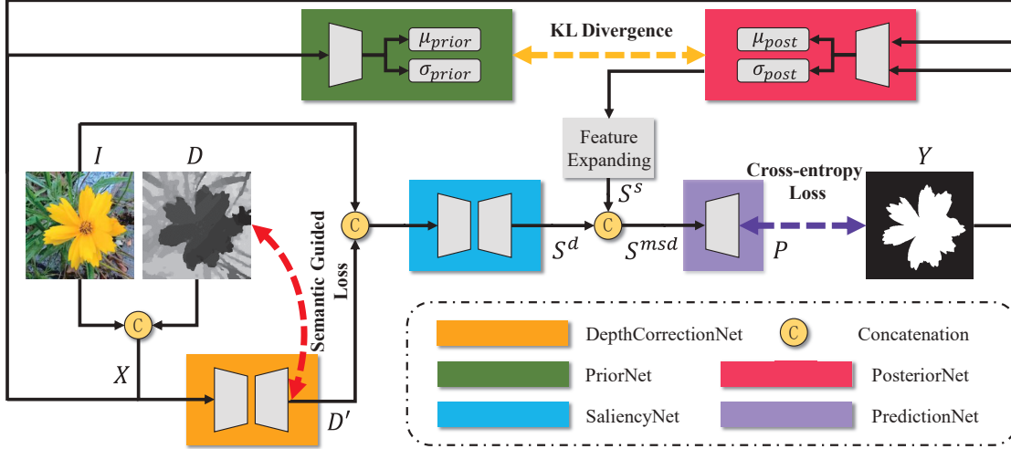
Figure 2. Network training pipeline. Four main modules are included, namely a LatentNet (PriorNet ( \mu_{prior}, \sigma_{prior} ) and PosteriorNet ( \mu_{post}, \sigma_{post} )), a SaliencyNet, a DepthCorrectionNet and a PredictionNet. The LatentNet maps the RGB-D image pair X (or together with GT Y for the PosteriorNet) to low dimensional Gaussian latent variable z . The DepthCorrectionNet refines the raw depth with a semantic guided loss. The SaliencyNet takes the RGB image and the refined depth as input to generate a saliency feature map. The PredictionNet takes both stochastic features and deterministic features to produce a final saliency map. We perform saliency consensus in the testing stage, as shown in Fig. 3 to generate the final saliency map according to the mechanism of GT saliency map generation.
