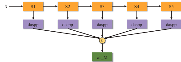
Figure 6. SaliencyNet, where “S1” represents the first stage of the VGG16 network, “daspp” is the DenseASPP module [58].
