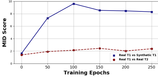
(a) DeepInversion [60]
