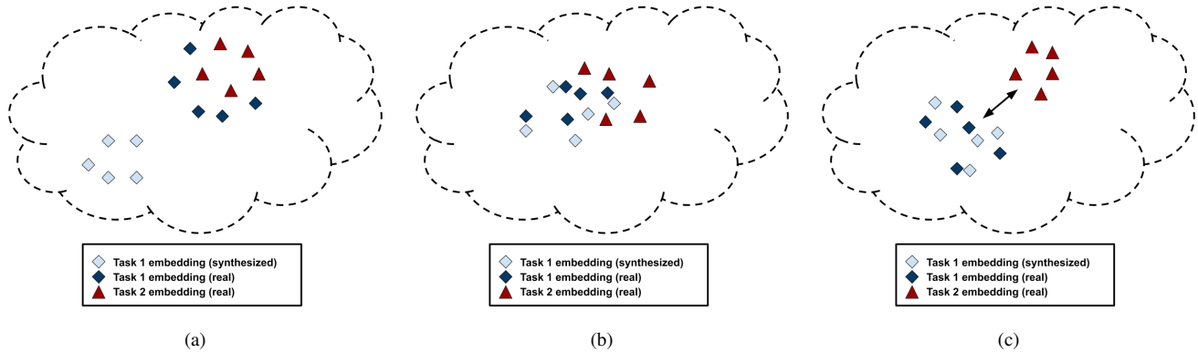
Figure 1: The distribution of feature embeddings when using synthetic replay data for class-incremental learning. (a) A straight application of synthetic data makes the model learn features more distinguishable between real and fake instead of task 1 and 2. This is the main problem analyzed and addressed in this work. (b) Modifying classification loss and adding regularization mitigates the feature drifting between real and fake. (c) This is the desired feature distributions. Our method makes task 1 and 2 more separable.
