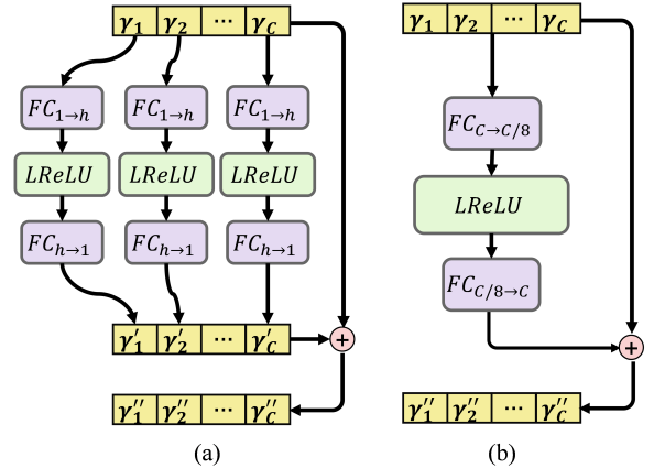
Figure 3. Details of (a) IERB and (b) CERB.
