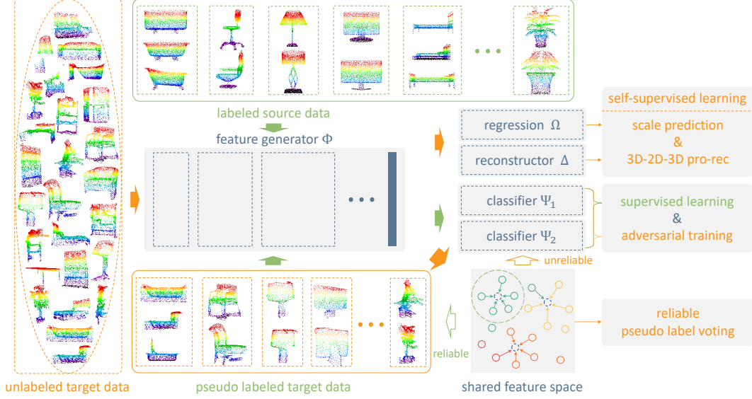
Figure 3. Illustration of the proposed self-supervised Global-Local structure modeling and Reliable Voted pseudo label method (GLRV) for point cloud domain adaption. The framework consists of a feature generator \Phi to encode point clouds, a regressor \Omega to predict the scaling change for self-supervised global structure modeling, a reconstructor \Delta to recover squeezed region for self-supervised local structure modeling and two classifiers \Psi_1 and \Psi_2 for supervised learning and adversarial training. Besides, a reliable voting method is employed to obtain accurate target pseudo labels for enhancing domain adaptation.
