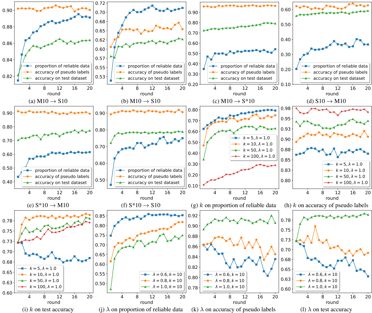
Figure 5. Influence of reliable voted pseudo labels. Experiments are conducted on PointDA. (a)~(f): With training, the proposed method adaptively selects more and more target data and test accuracies increase gradually. (g)~(l): Impact of k and \lambda on voted pseudo label generation and adaptation performance ( S^*10 \rightarrow S10 ). To show the real trend, test accuracies are evaluated without source validation.
