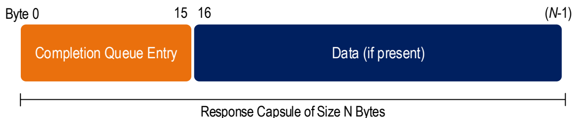
Figure 82: Response Capsule
