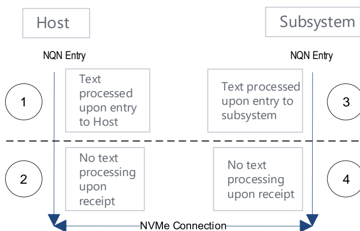
Figure 138: NQN Processing
