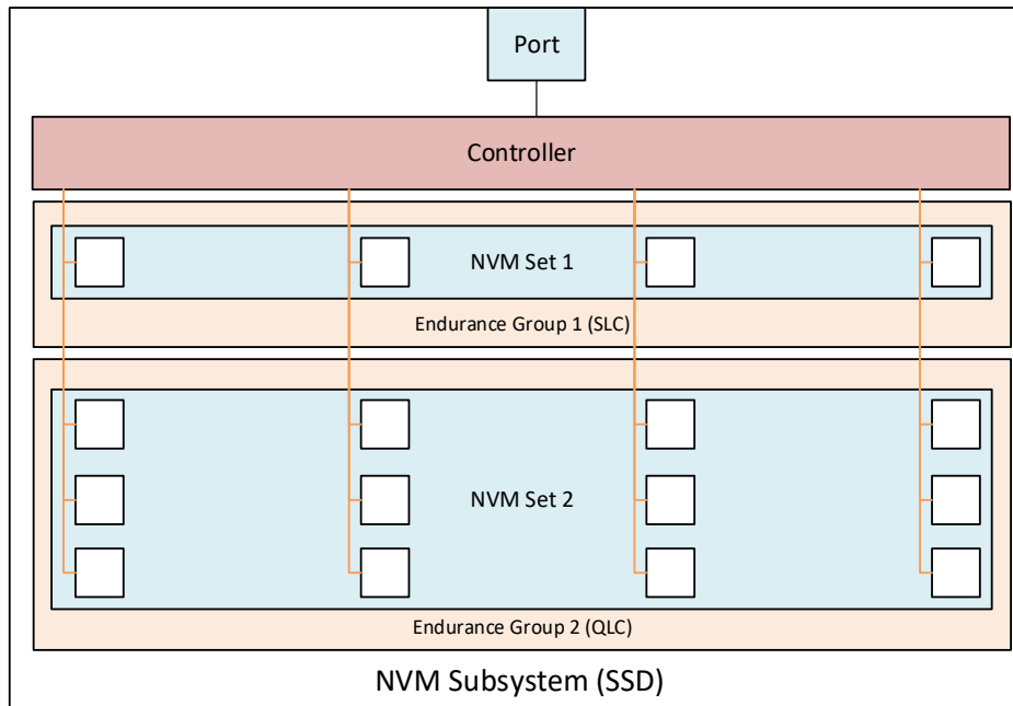
Figure 108: Horizontally-Organized Dual NAND NVM Subsystem
