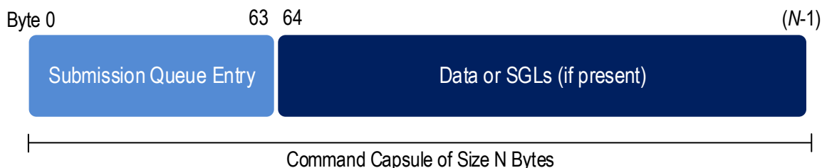
Figure 79: Command Capsule
