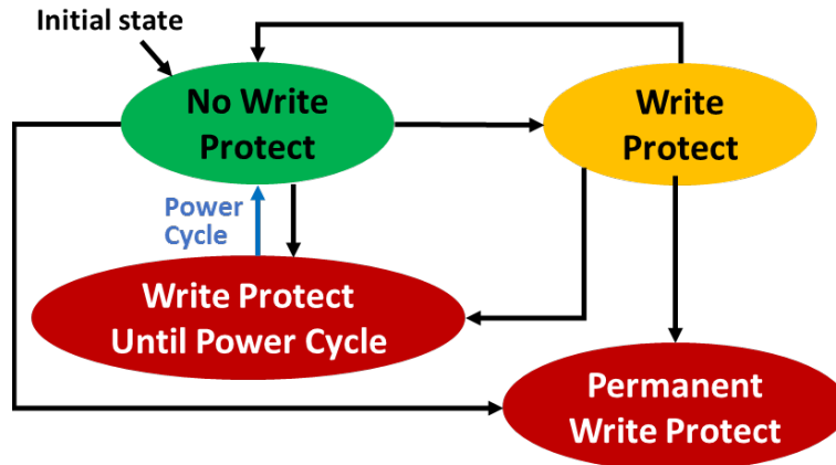
Figure 491: Namespace Write Protection State Machine Model
