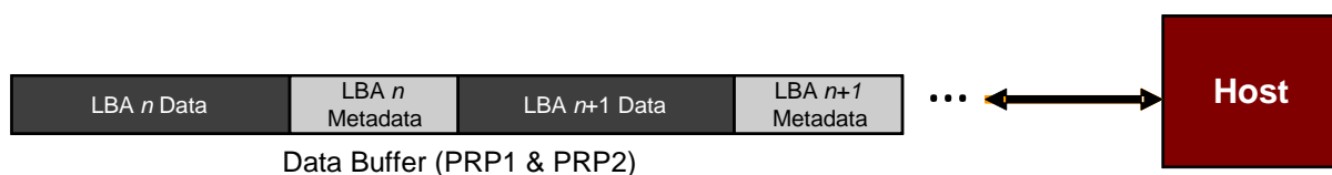
Figure 451: Metadata – Contiguous with LBA Data, Forming Extended LBA
