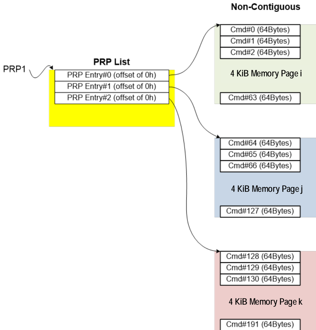
Figure 435: PRP List Describing I/O Submission Queue
