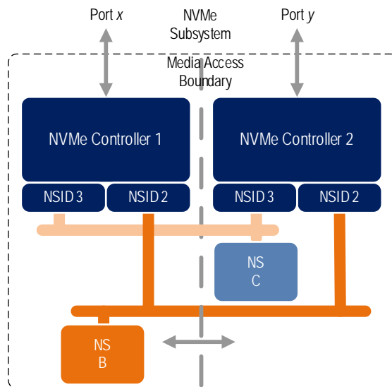
Figure 494: Namespace B optimized through Controller 1
