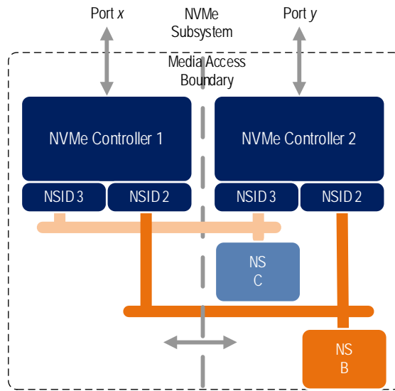
Figure 493: Namespace B and C optimized through Controller 2
