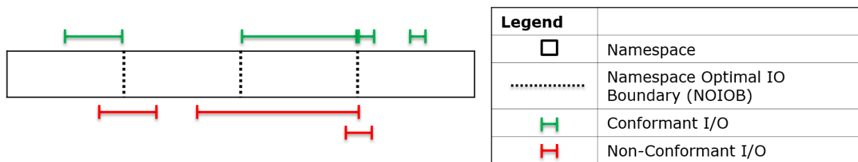
Figure 501: An example namespace with four NOIOBs
