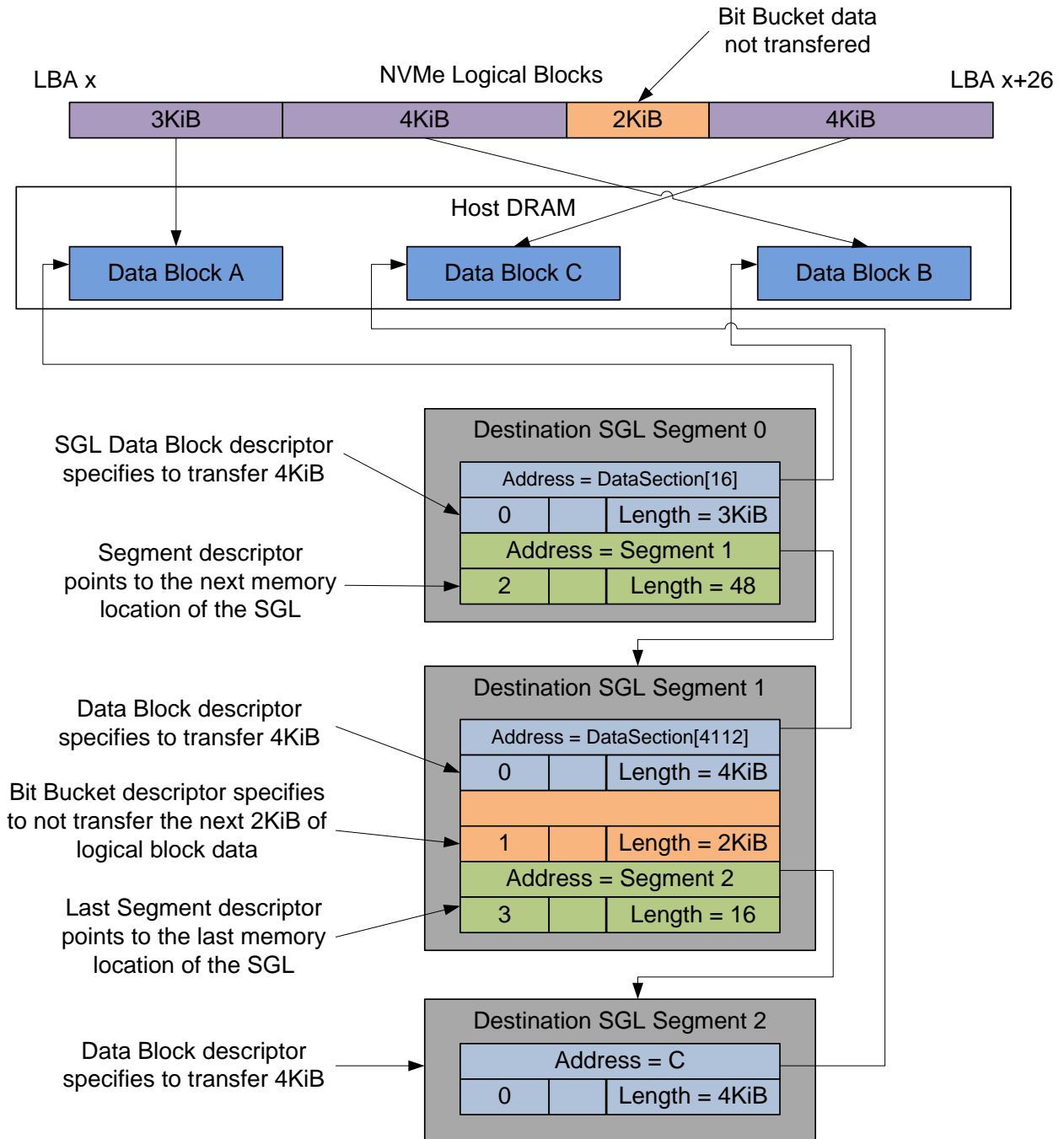
Figure 121: SGL Read Example
