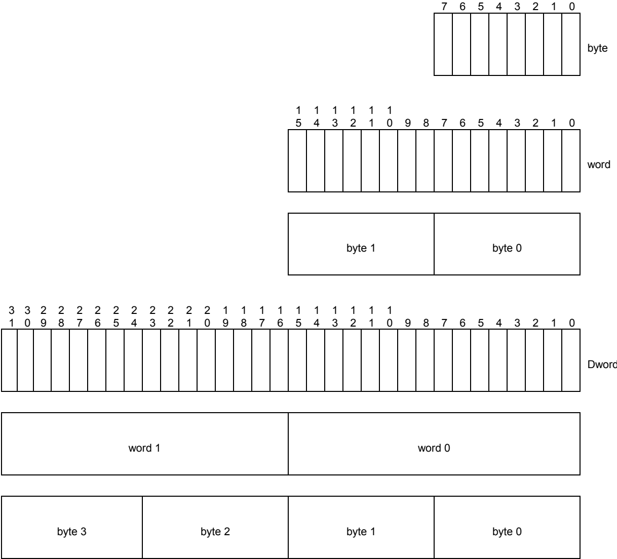
Figure 3: Byte, word and Dword Relationships
