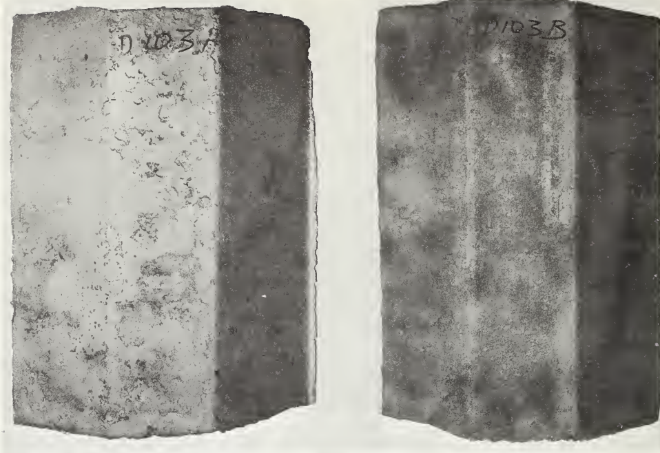
FIGURE 3. Sections (1.5 ft by 1 ft) cut from a piling which was pulled from the north upstream wingwall of the Grenada Dam Spillway at Grenada, Mississippi, after exposure for 12 years.
