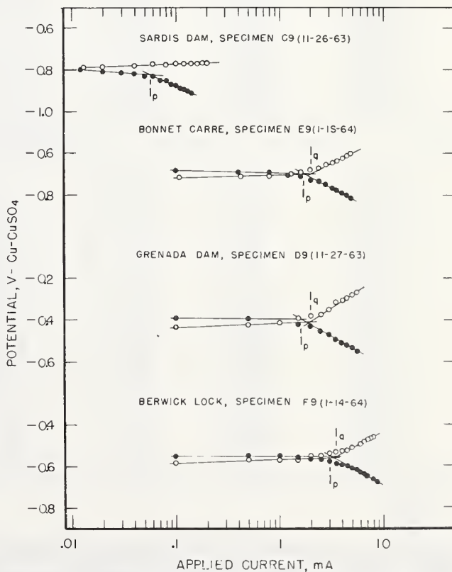
FIGURE 3. Polarization curves of underground specimens Nos. 9 after 45 months of exposure at four soil sites.
