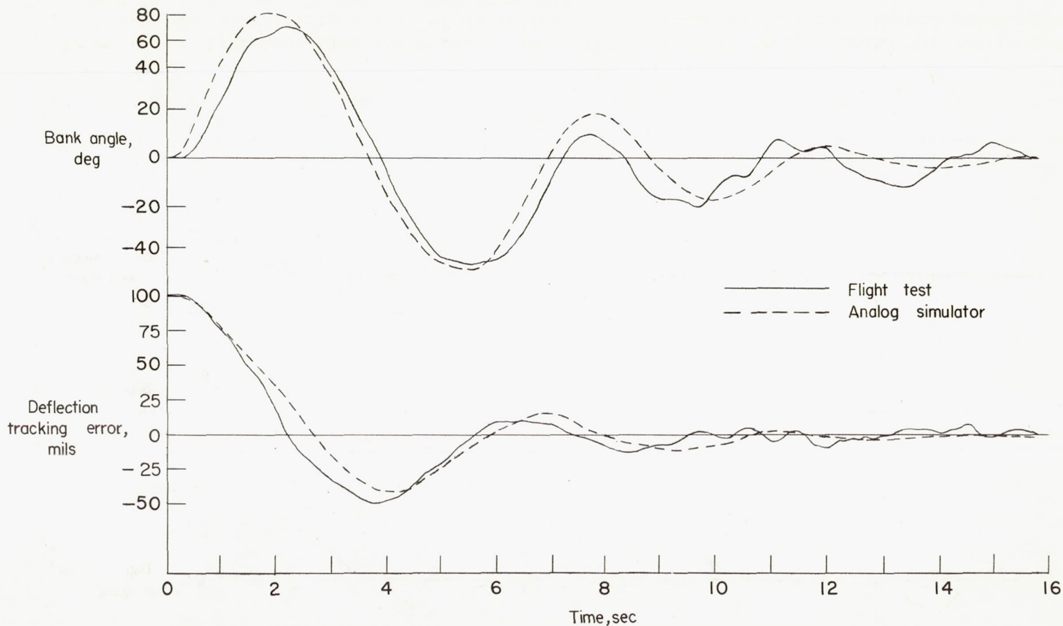
Figure 11.- Time histories from a flight-test run and an analog-simulator run illustrating similarity of results from these tests. Approximately the same gains were used in both runs. The radar-boresight axis was oriented 1/2^\circ above the armament-datum line for the flight-test system and coincident with the roll axis for the analog-simulator system.
