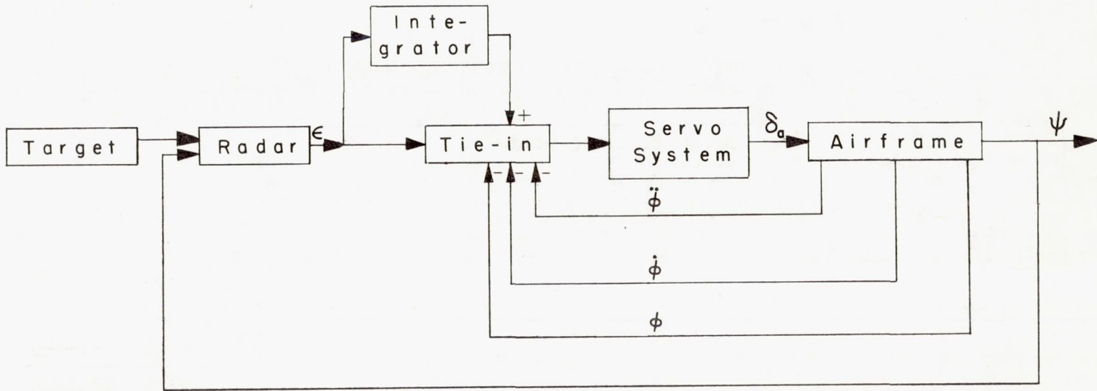
Figure 3.- Schematic diagram of deflection channel of automatic interceptor system.
