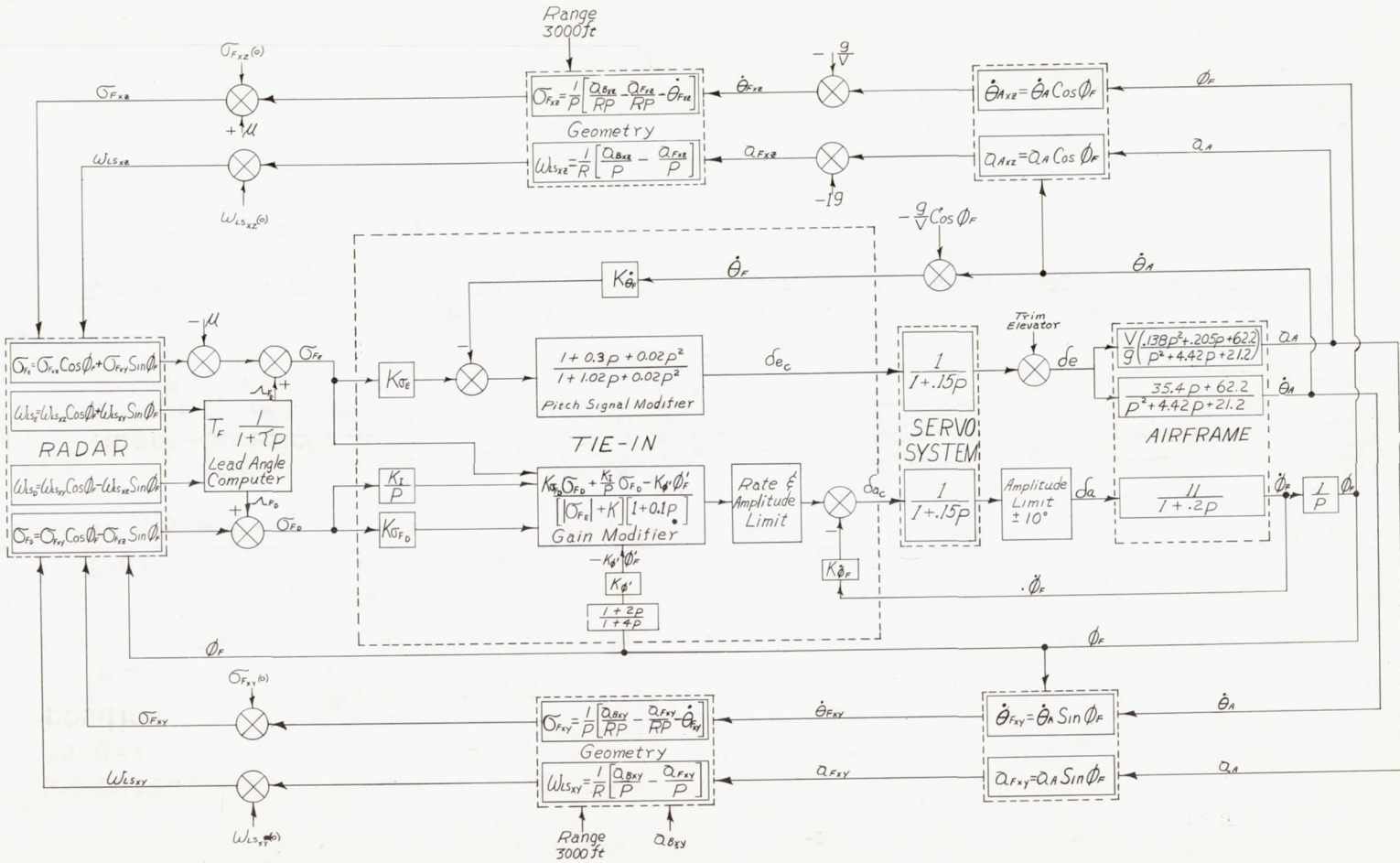
Figure 7.- Schematic of automatic-interceptor problem as set up on analog simulator.
