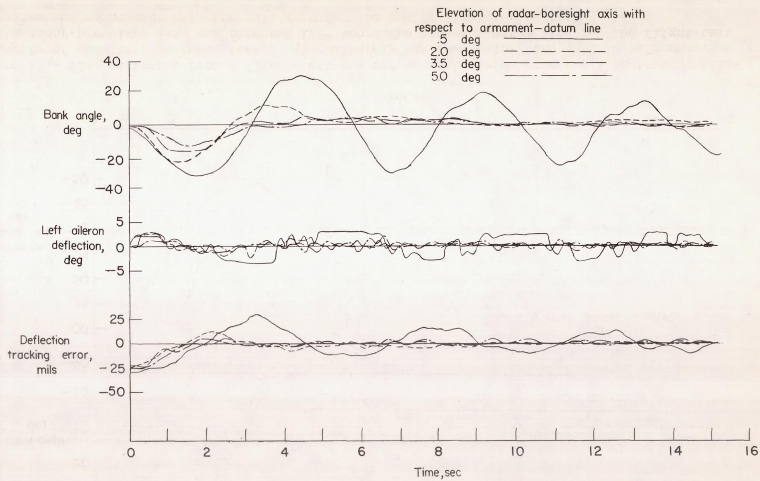
Figure 12.- Flight-test time histories of interceptor response to an initial deflection error showing the stabilizing effect of elevating the radar-boresight axis. Normal gains were used in each case. Target is nonmaneuvering.
