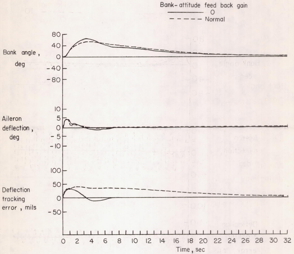
Figure 20.- Time histories from analog-simulator run where interceptor began attack from 30° off target tail showing beneficial effect of eliminating bank-attitude feedback. Range equals 7,000 feet.
