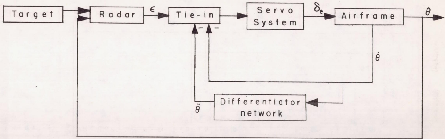
Figure 2.- Schematic diagram of elevation channel of automatic interceptor system.
