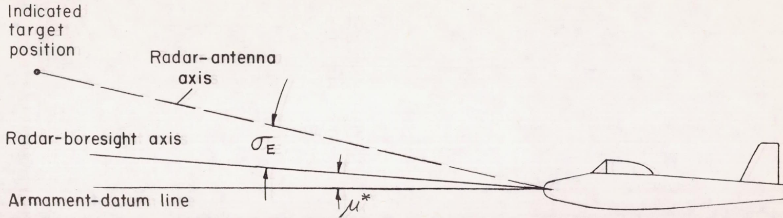
Figure 6.- Diagram of relationship between automatically controlled interceptor axis system where no deflection tracking error exists. (Applies to flight tests without lead angles.)
