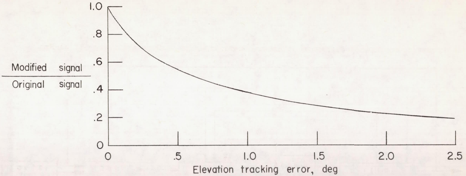
Figure 4.- Modification of deflection tracking-error signal and roll-attitude feedback signal effected in tie-in.
