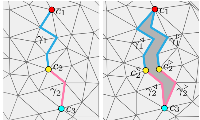
Fig. 4. The cutting scheme used in this paper. Left: the 3 vertices selected as cones are connected with two edge-paths; right: cutting the mesh through the paths duplicates vertices and edges along the cut into corresponding copies.
