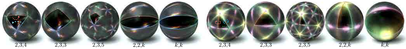
Fig. 2. The different orbifolds used in this paper, visualized by tiling the sphere with copies of the representative basic tile (in bold color). On the left are the 5 orbifolds with rotational symmetry and sphere-like topology, on the right, the 5 orbifolds with reflectional symmetry and disk-like topology.
