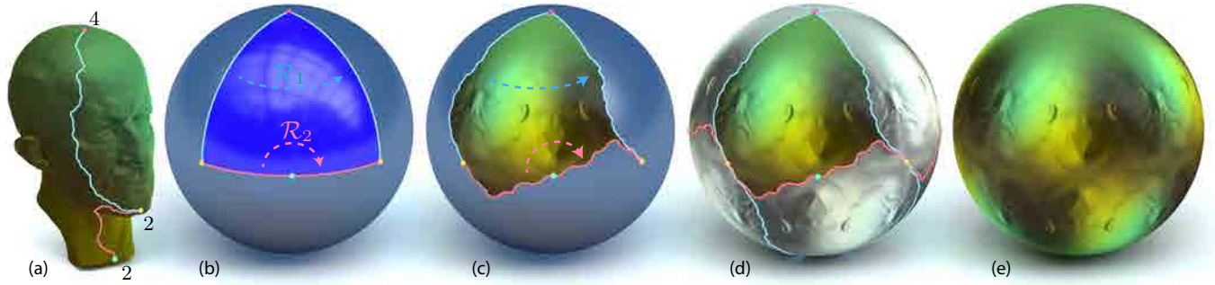
Fig. 3. The outline of our method. (a) the input to our algorithm consists of an input mesh and a discrete set of cones (in this case there are 3, visualized as colored balls) and an integer n_i associated to each cone denoting its symmetry-order. (b) according to the number of cones and their order, we construct a basic tile describing the boundary conditions of the embedding; in this specific tile, the two blue edges are associated by a 90^\circ rotation, \mathcal{R}_1 , and the two red edges are associated by a 180^\circ rotation, \mathcal{R}_2 . (c) the output of our algorithm – an embedding of the cut mesh into the sphere, which minimizes the spherical Dirichlet energy under the boundary conditions defined according to the basic tile. (d) the specific boundary conditions ensure that we can tile the entire sphere with rotated copies of the embedding – this is the special symmetry property of an orbifold embedding. The resulting tiled embedding is a bijective, discrete harmonic and (as shown in (e)) seamless embedding into the orbifold. The number of rotated copies of the mesh around each cone respects the symmetry order associated to the cone.
