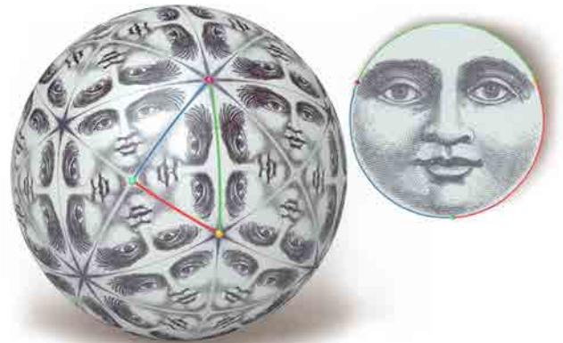
Fig. 10. An embedding of a flat disk mesh to a disk-like orbifold with reflective cones of order 4, 3, 2.
