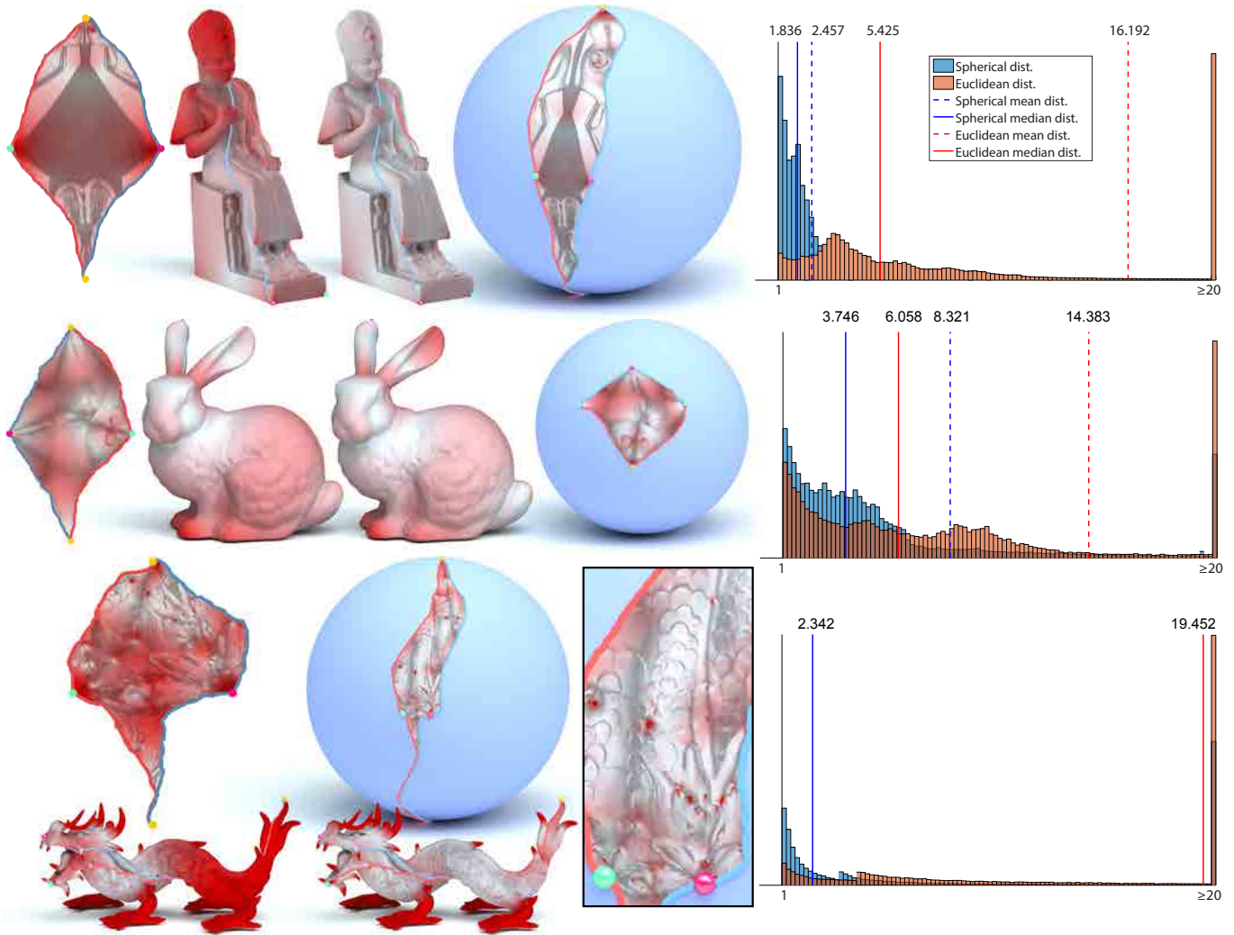
Fig. 12. Comparison of the spherical orbifold Tutte embeddings (to the right in each row) to the Euclidean orbifold Tutte embeddings (to the left in each row). Both methods produce conformal maps, however the spherical orbifolds enable generating embeddings with lower area distortion (meshes colored according to distortion). The histogram of the distortion is shown next to each example.
