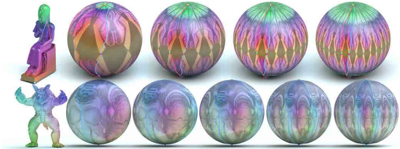
Fig. 7. Top: an embedding of a sphere-like mesh to a 3-cone sphere orbifold with cones of order 2, 2, k , where k can be any integer larger than 1; we show k = 4, 8, 12, 16 . Bottom: an embedding of a sphere-like mesh to a 2-cone sphere orbifold, where the two cones are placed at the north and south poles and have the same order k . The results shown are for k = 2, 3, 4, 6, 8 .
