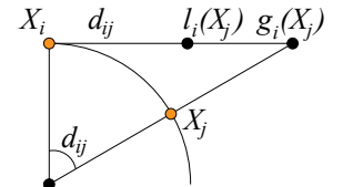
Fig. 5. Inverse exponential and gnomonic projections.
