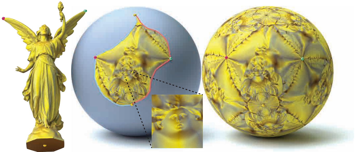
Fig. 1. A spherical orbifold Tutte embedding: a mesh (left) is embedded to a tile on the sphere (middle), which generates a seamless tiling of the entire sphere (right). Three points (visualized as colored balls) are designated as cones – symmetry points of the tiling.
