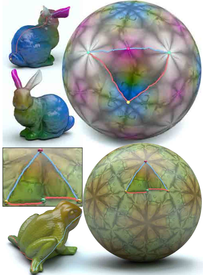
Fig. 6. Embeddings of sphere-like meshes to sphere-like orbifolds with cones of order 4, 3, 2 (top) and 5, 3, 2 (bottom).
