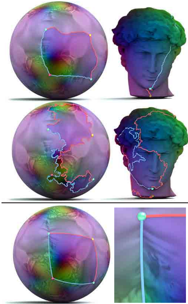
Fig. 13. Our embedding is seamless, and is only affected by the choice of cones, as shown in the top two rows: we modify the cuts on the mesh (without modifying the cone placement) and produce two embeddings – although they generate two different tiles (in bold color, left column), after tiling the results are identical and in fact represent the same orbifold embedding. In the bottom row, we show the embedding we initialize our optimization with, which, as can be seen in the blowup, is affected by the placement of the cuts.
