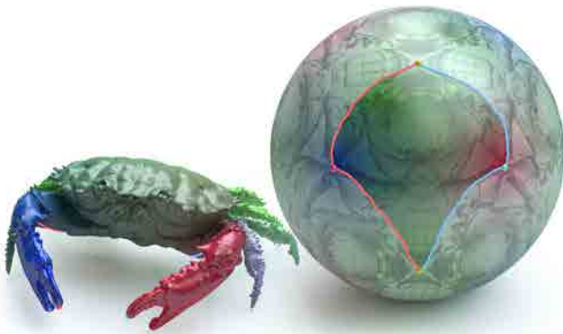
Fig. 8. An embedding of a sphere-like mesh of 2M triangles to a sphere-like orbifold with cones of order 3, 3, 2.
