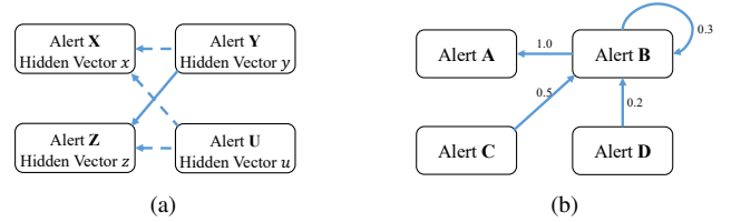
Fig. 6. The dotted/solid lines in Fig. 6a indicate the fake/real causality links. Fig. 6b shows self-loop attention and normalization.
