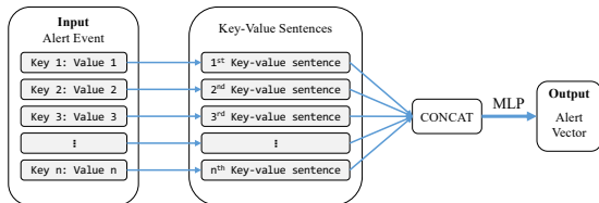
Fig. 5. Workflow of the Alert2Vec module.
