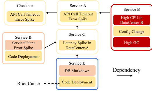
Fig. 2. Illustration of service dependency graph, where an alert in Service E is the ground-truth root cause.
