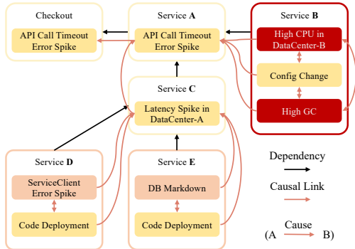
Fig. 4. An example of Alert Dependency Graph
