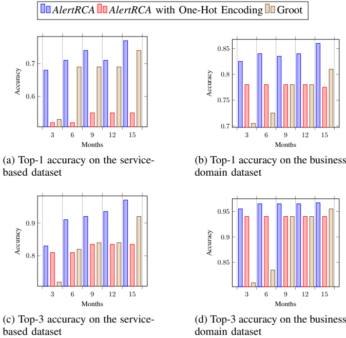
Fig. 7. Performance of AlertRCA , AlertRCA with one-hot encoding, and Groot.
