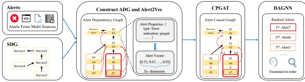
Fig. 3. The workflow of AlertRCA . S1 and A1 are abbreviations for Service 1 and Alert 1, respectively.
