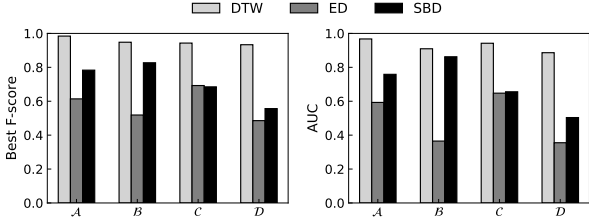
(b) Comparison with different distance measures.
