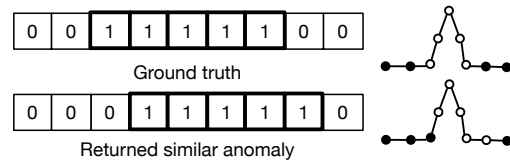
Fig. 7: Illustration of true positive. Anomaly is denoted by 1 and marked in hollow point on the right. The first row is the ground truth with an anomaly segment highlighted in shaded squares. The returned similar anomaly shown in the second row has a more than 50% overlap with labeled anomaly in truth. Hence, we regard it is a true positive.
