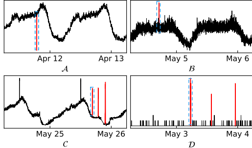
Fig. 6: 2-day-long fragments of the KPIs in our datasets. Similar anomalies are labeled in red color and the anomaly templates are marked in blue dashed rectangles.
