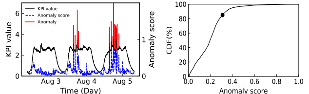
(b) Comparison of anomaly scores (c) The CDF of anomaly scores between normal points and anomalies. The black point is 85 th percentile.
