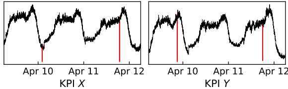
Fig. 1: Similar anomalies (labeled in red) in KPIs X and Y . similarity search , which given an anomaly template by the operator, i.e. , a KPI segment containing known anomalous data points, discovers anomalies similar to the template among the candidate anomalies.
