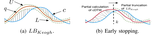
Fig. 5: Illustration of LB_{Keogh} and early stopping of DTW, adopted and slightly modified from Figure 6 in [21].
