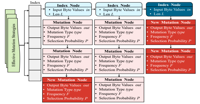
Fig. 4: The data structure of PBOM .
