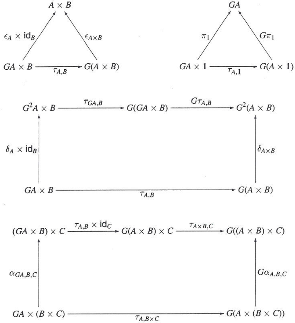
Figure 8: Requirements for a strong comonad
