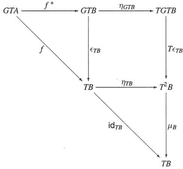
Figure 13: Proof that \epsilon'_B \overset{T}{\circ} f^{+'} = f .
