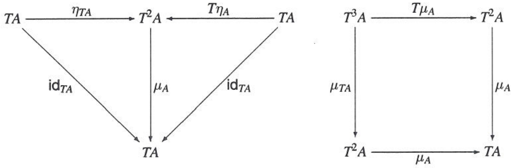
Figure 1: Identity and Associativity laws for a monad
