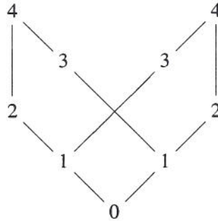
Figure 10: Definition of f on A
