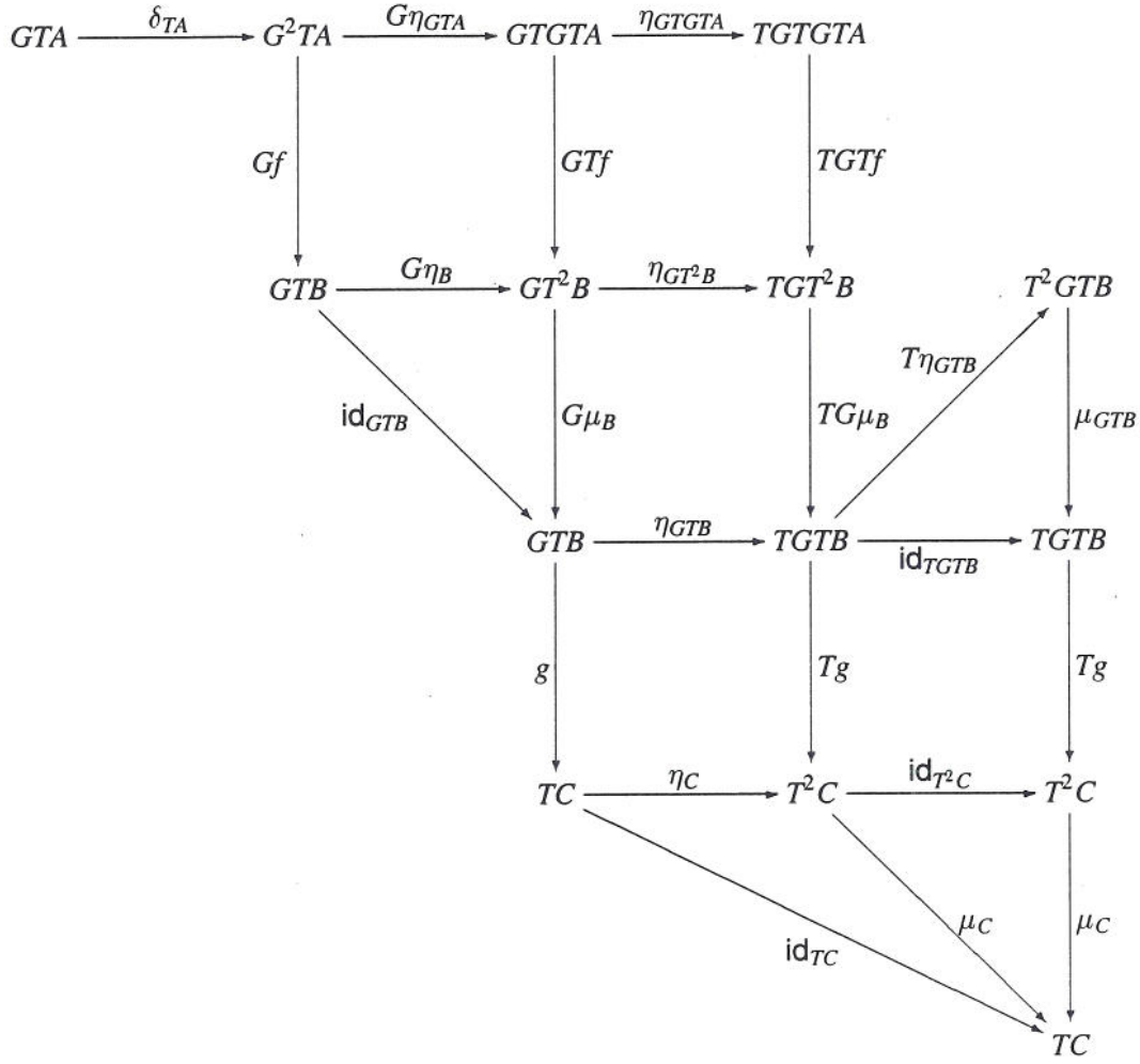
Figure 14: Proof that g \overset{T}{\circ} G'f \overset{T}{\circ} \delta'_A = g \circ Gf \circ \delta_{TA} . The upper part of the diagram represents g \overset{T}{\circ} (G'f \overset{T}{\circ} \delta'_A) = \mu_C \circ Tg \circ \mu_{GTB} \circ T\eta_{GTB} \circ TG\mu_B \circ TGTf \circ \eta_{GTGTA} \circ G\eta_{GTA} \circ \delta_{TA} .
