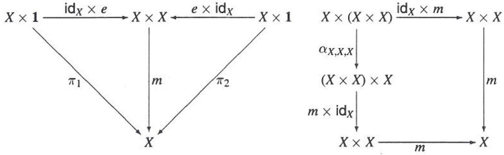
Figure 2: Identity and Associativity properties of a monoid
