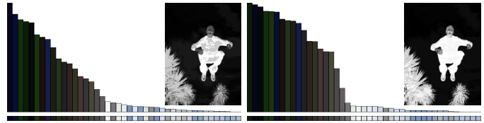
Fig. 4. Saliency of each color before (left) and after (right) color space smoothing. Corresponding saliency maps are shown in the respective insets.
