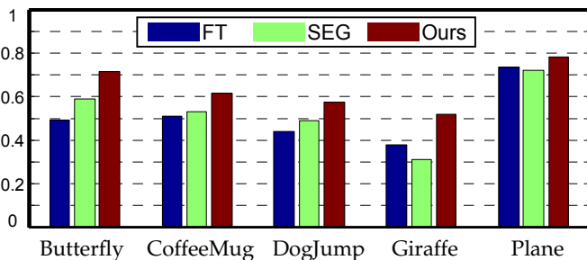
Fig. 13. Comparison of average F_{\beta} for different saliency segmentation methods: FT [33], SEG [25], and ours, on THUR15K dataset [51].
