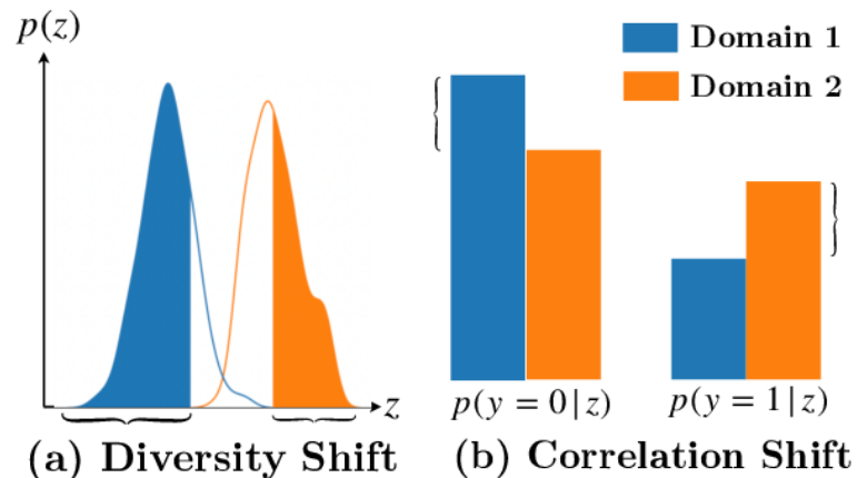
Figure 17.28.: The curly brackets enclose the distribution shift between the environments. Here, z stands for the spurious feature, and y stands for label class. Source: Xin
