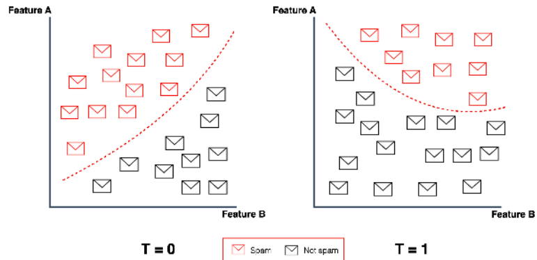
Figure 17.29.: Concept drift refers to a change in data patterns and relationships over time. Source: Evidently AI
