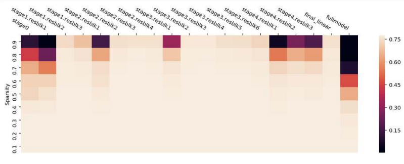
Figure 9.40.: Sparse network heat map. Source: Numenta.
