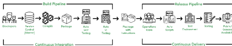
Figure 17.37.: Continuous Integration/Continuous Deployment (CI/CD) procedure. Source: geeksforgeeks
