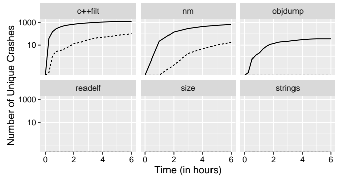
Fig. 9. Average #crashes over time (on a log-scale) for AFLFAST (solid line) vs. AFL (dashed line) computed as mean over all runs in five minute intervals.
