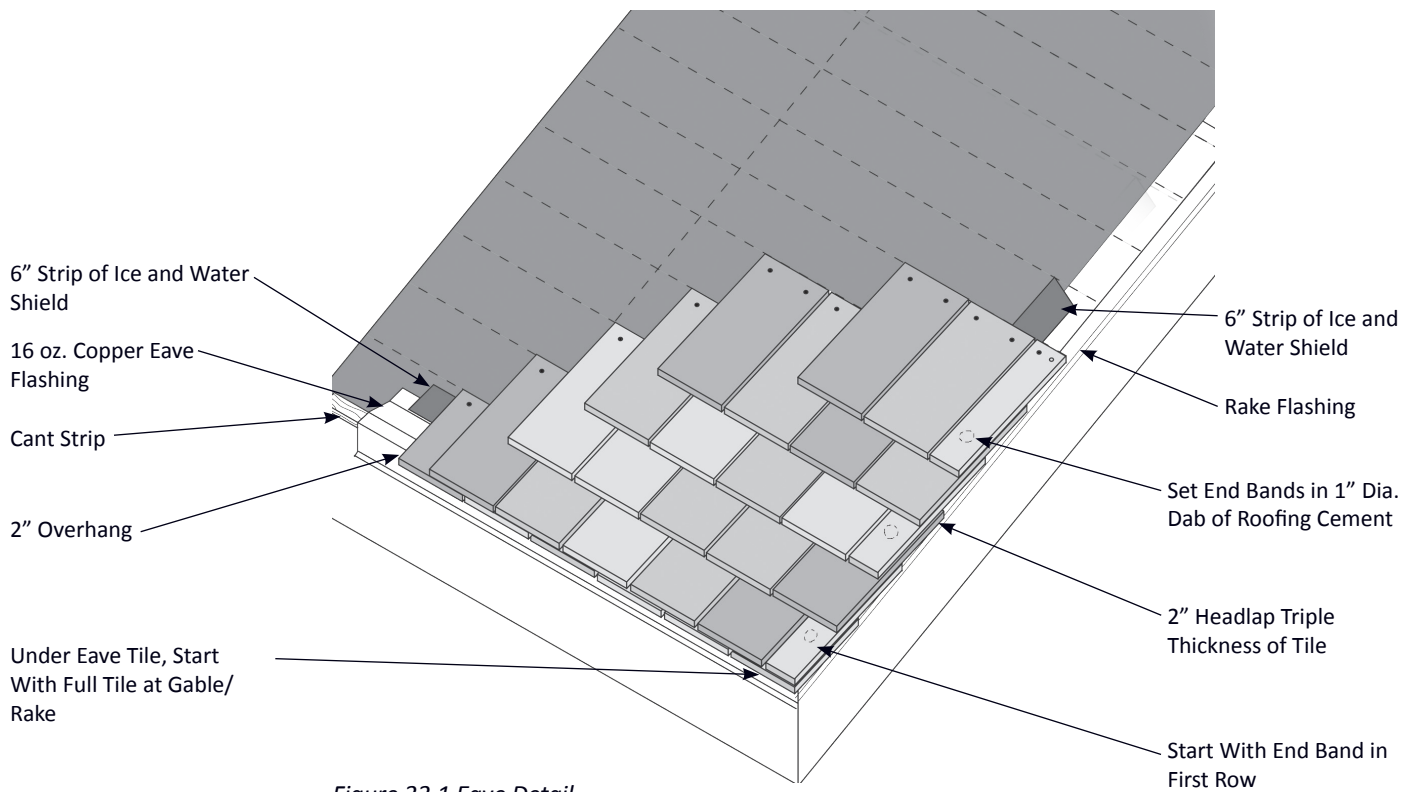
Figure 33.1 Eave Detail
