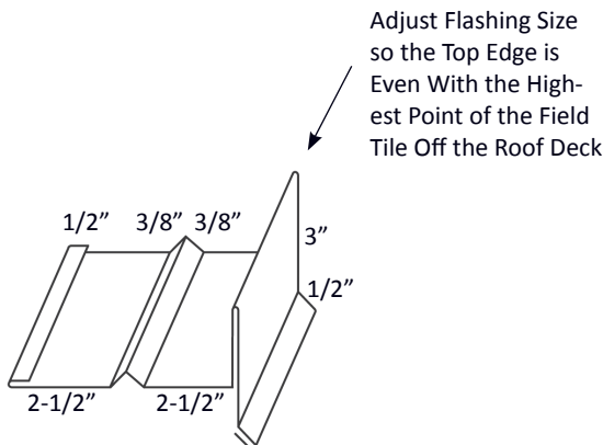
Figure 23.2 Closed Rake Flashing Dimensions
