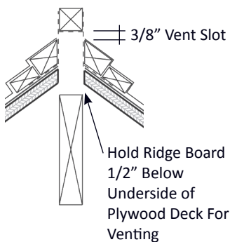
Figure 39.3 Vented Circular Cover Framing
