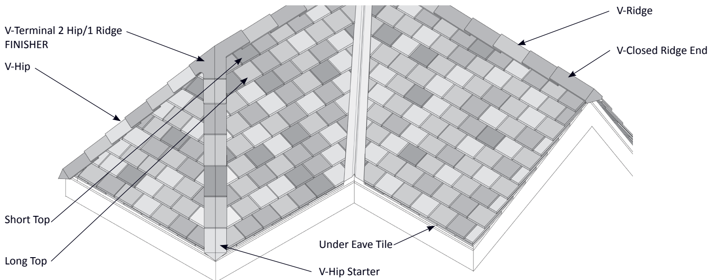
Figure 32.1 Shingle Tile
