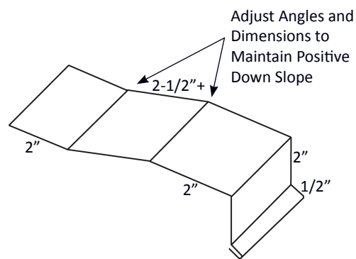
Figure 22.1 Eave Flashing Dimensions
