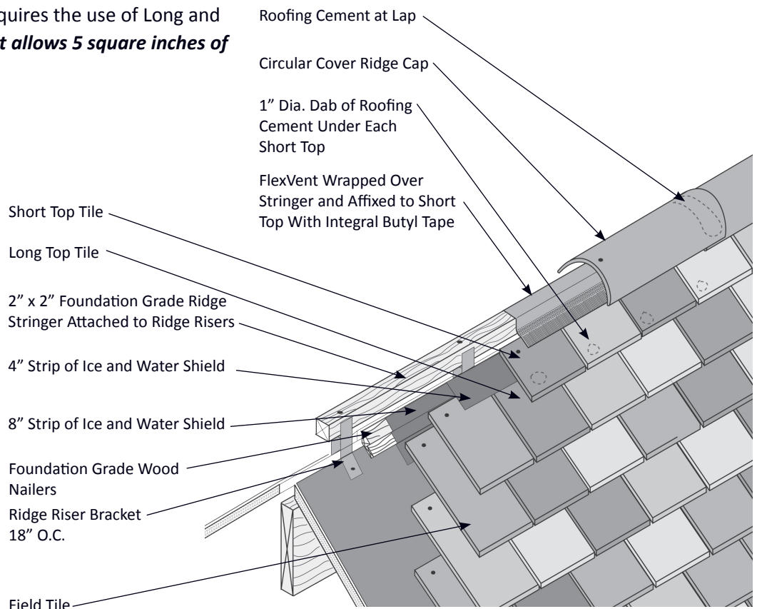
Figure 39.2 Vented Circular Cover Ridge Detail
