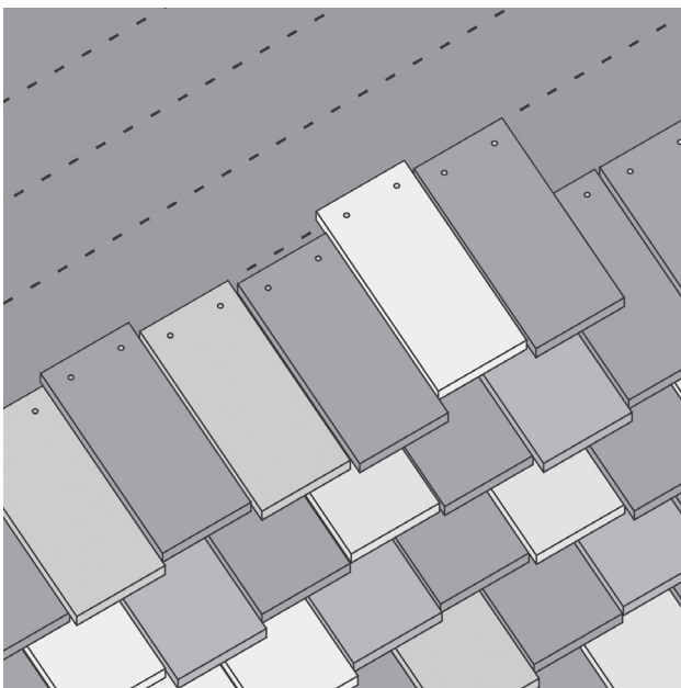
Figure 42.3 Staggered Layout
