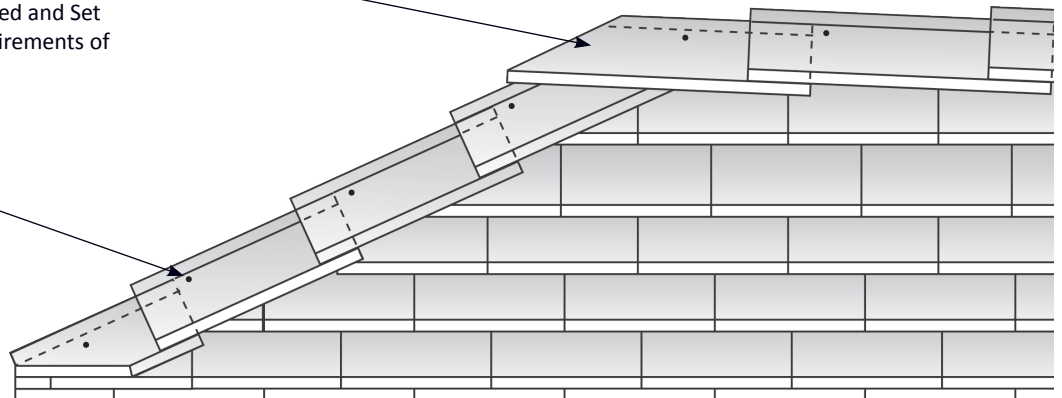
Figure 37.2 Saddle Hip & Saddle Ridge Terminal
