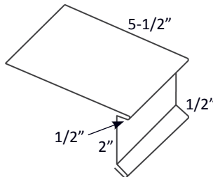
Figure 23.1 Open Rake Flashing Dimensions
