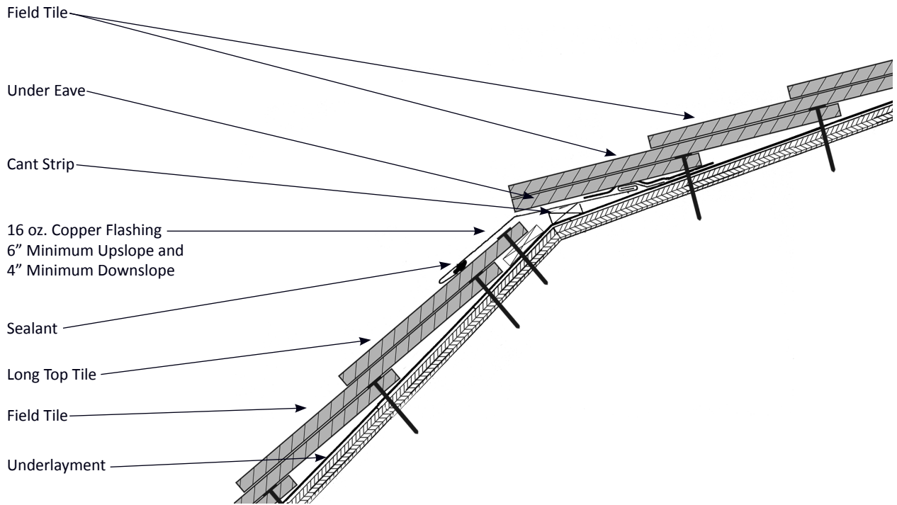
Figure 31.1 Flashing at High Slope to Low Slope Transition
