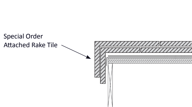
Figure 23.5 Attached Rake Detail
