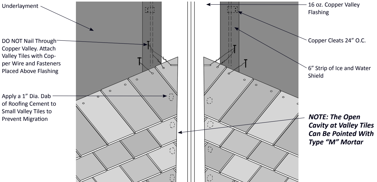
Figure 34.1 Valley Detail
