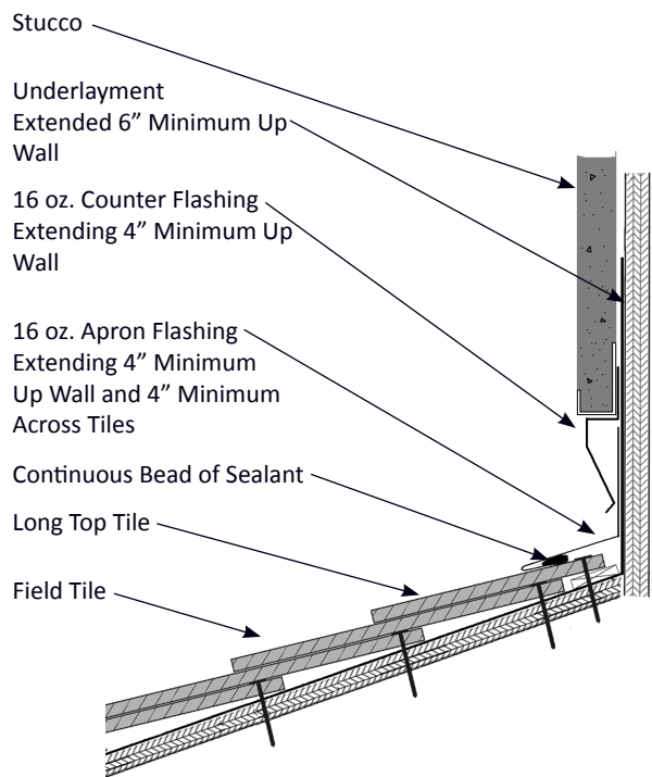
Figure 28.2 Counter Flashing & Apron Flashing at Head Wall
