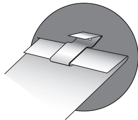
Figure 24.3 Copper Cleat Detail
