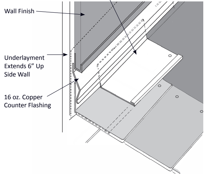
Figure 26.2 Side Wall Copper Step Flashing With Counter Flashing
