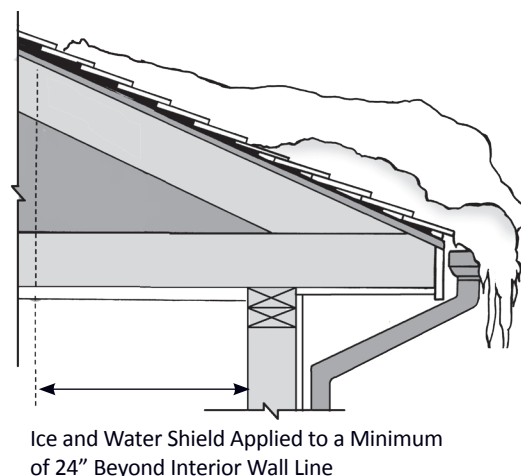
Figure 14.2 Ice Dam Protection
