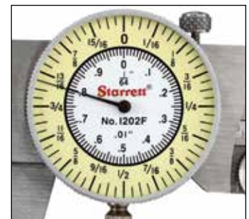
Dial displays both fractional and decimal measurements
