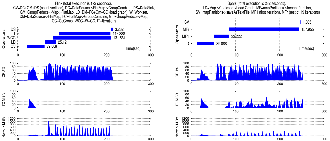
Fig. 16: Page Rank resource usage of Flink and Spark for 27 nodes, 20 iterations, Small Graph. Disk utilization is similar to disk I/O, memory is 40%.
