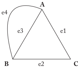
Figure 17.9. Example of a Multigraph
