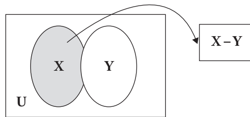
Figure 17.6. Venn Diagram for X - Y
