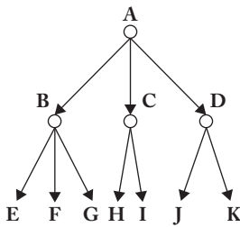
Figure 17.15. Example of a Tree
