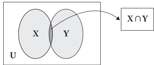
Figure 17.3. Intersection of Sets X and Y
