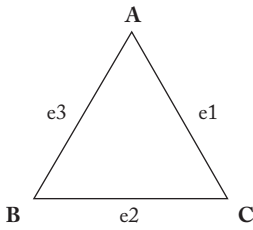
Figure 17.8. Example of a Graph
