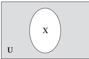
Figure 17.5. Venn Diagram for Complement Set of X
