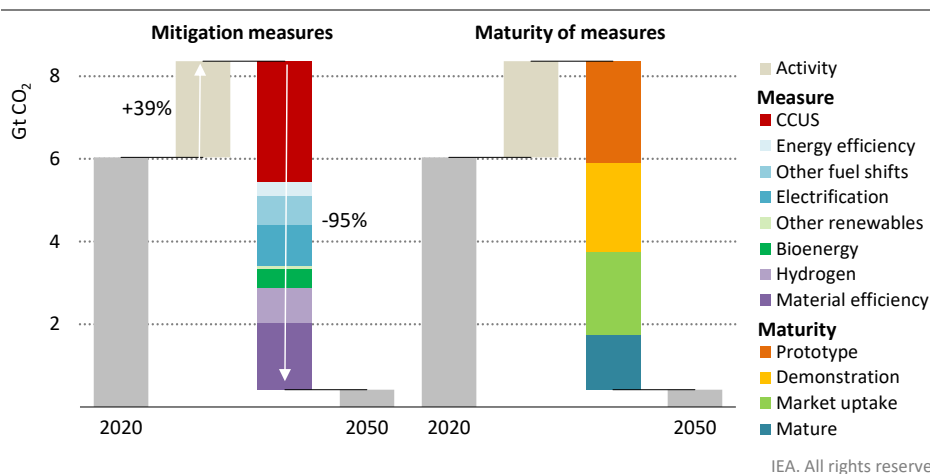
Figure 3.16 ▶ Global CO 2 emissions in heavy industry and reductions by mitigation measure and technology maturity category in the NZE
