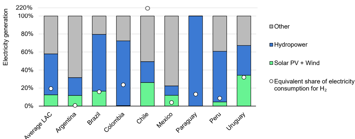
Figure 8.7 Potential electricity demand for electrolytic hydrogen production from announced projects in Latin America and the Caribbean, 2030, and electricity generation, 2022
