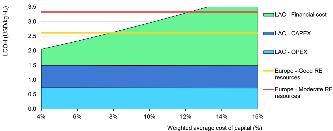
Figure 8.22 Impact of cost of capital on hydrogen production costs in Latin America and the Caribbean vs Europe in the Announced Pledges Scenario, 2030
