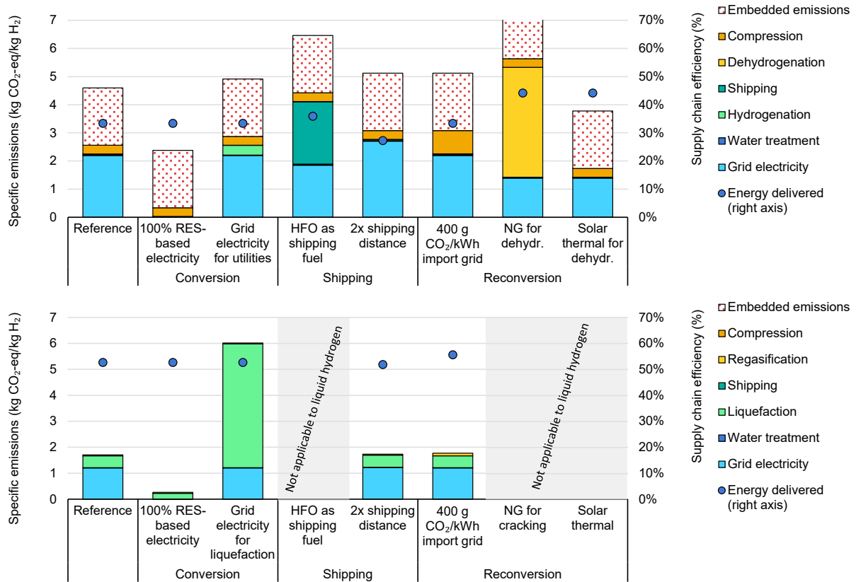
Figure 7.8 GHG emissions intensity for liquid organic hydrogen carrier (top) and liquid hydrogen (bottom) supply chains
