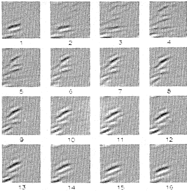
Fig. 25. The scalar-sensor responses R_{h,l} to the input in Fig. 24. Scale, 8 cycles/width, direction, 108^\circ . The first four frames are wrap-arounds from the end of the response.
