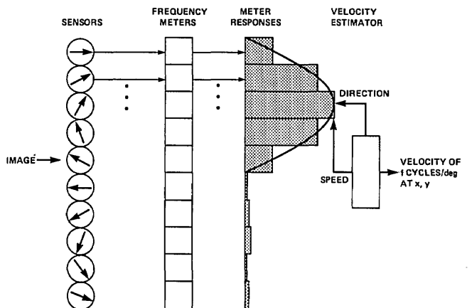
Fig. 13. The structure of the vector motion sensor.
