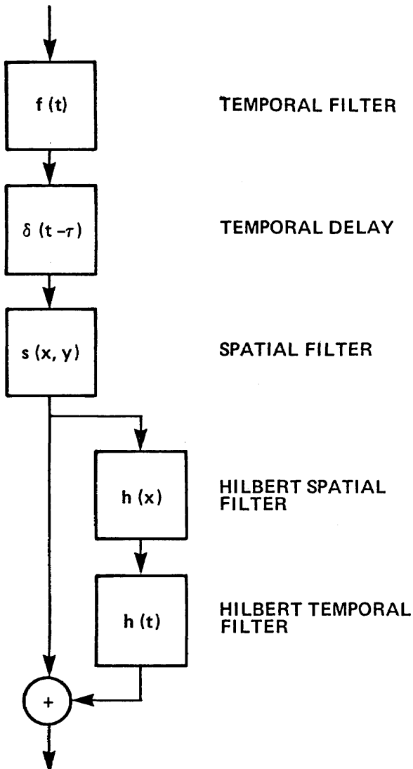
Fig. 4. Mathematical structure of the scalar motion sensor.
