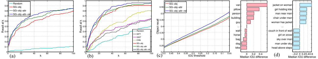
Figure 7: (a) Retrieval performance for entire scenes, (b) for partial scenes. (c) Object localization performance for entire scenes. (d) Increase in localization performance of our full model SG-obj-attr-rel vs SG-obj for individual objects (left) and objects participating in a relation (right). In (d), positive values indicate the SG-obj-attr-rel performs better than SG-obj.
