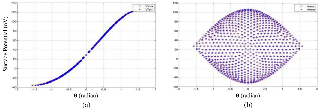
Figure 6. Analytical ( ^{\circ} Vana) and numerical solution (*Vfem) on all surface's nodes versus the theta angle (radian), (b) shows the result for a centered radial dipole, (a) those for a centered tangential dipole.
