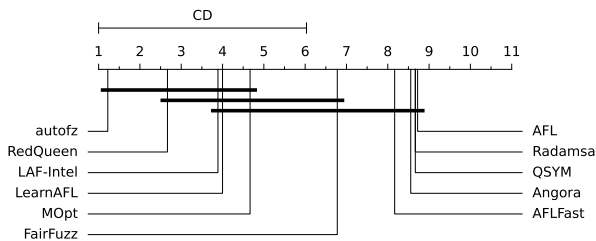
Figure 4: Critical Difference for the targets in UNIFUZZ. Each number indicates the average rank of fuzzers. Each bold line indicates that there is no statistical difference in performance among the fuzzers grouped by that line in terms of the Nemenyi post-hoc test.
