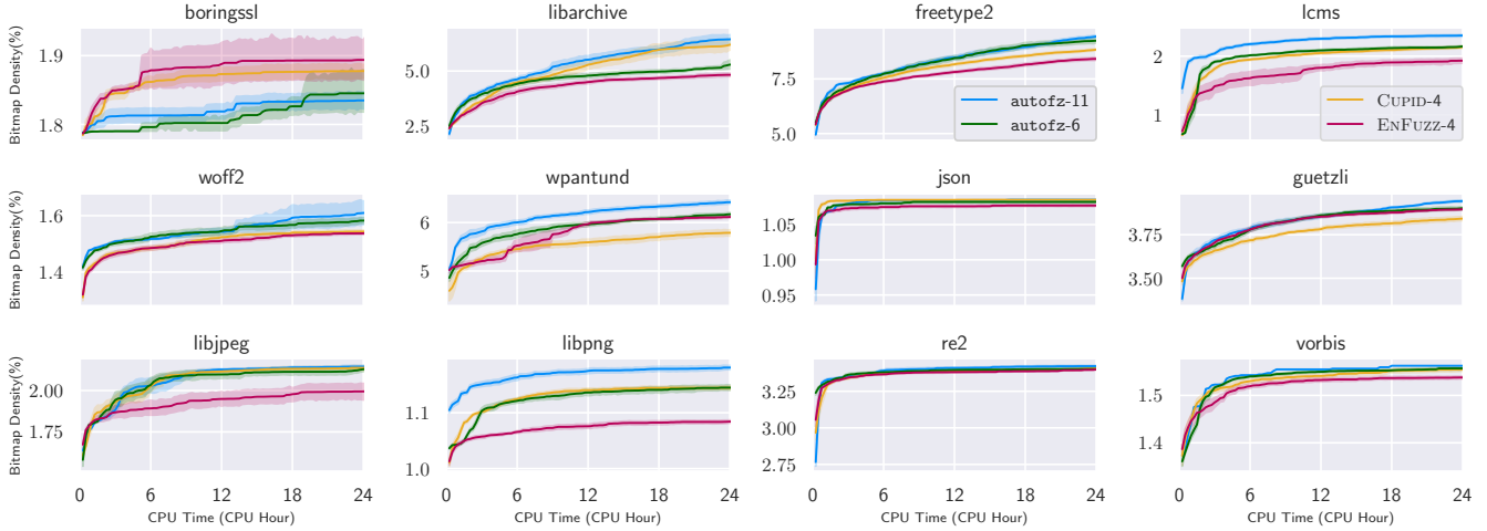
Figure 11: Comparison among autofz, ENFUZZ, and CUPID. Each line plot is depicted with an arithmetic mean and 80% confidence interval for 10 times fuzzing runs. The coverage ratio is a percentage of branches explored by each fuzzer. X-axis is elapsed CPU time . Below is the list of fuzzers used by different configurations: autofz-6 = [AFL, FairFuzz, QSYM, AFLFast, libFuzzer, Radamsa ], CUPID-4 = [AFL, FairFuzz, QSYM, libFuzzer ], ENFUZZ-4 = [AFL, FairFuzz, Radamsa, libFuzzer ] which is reported to be the best in [11], autofz-11 = [All baseline fuzzers described in §6]
