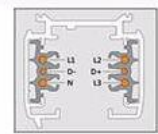
6 wires Track
