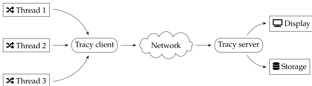
Figure 2: Client-server model.
