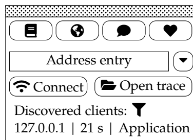
Figure 9: Welcome dialog.
