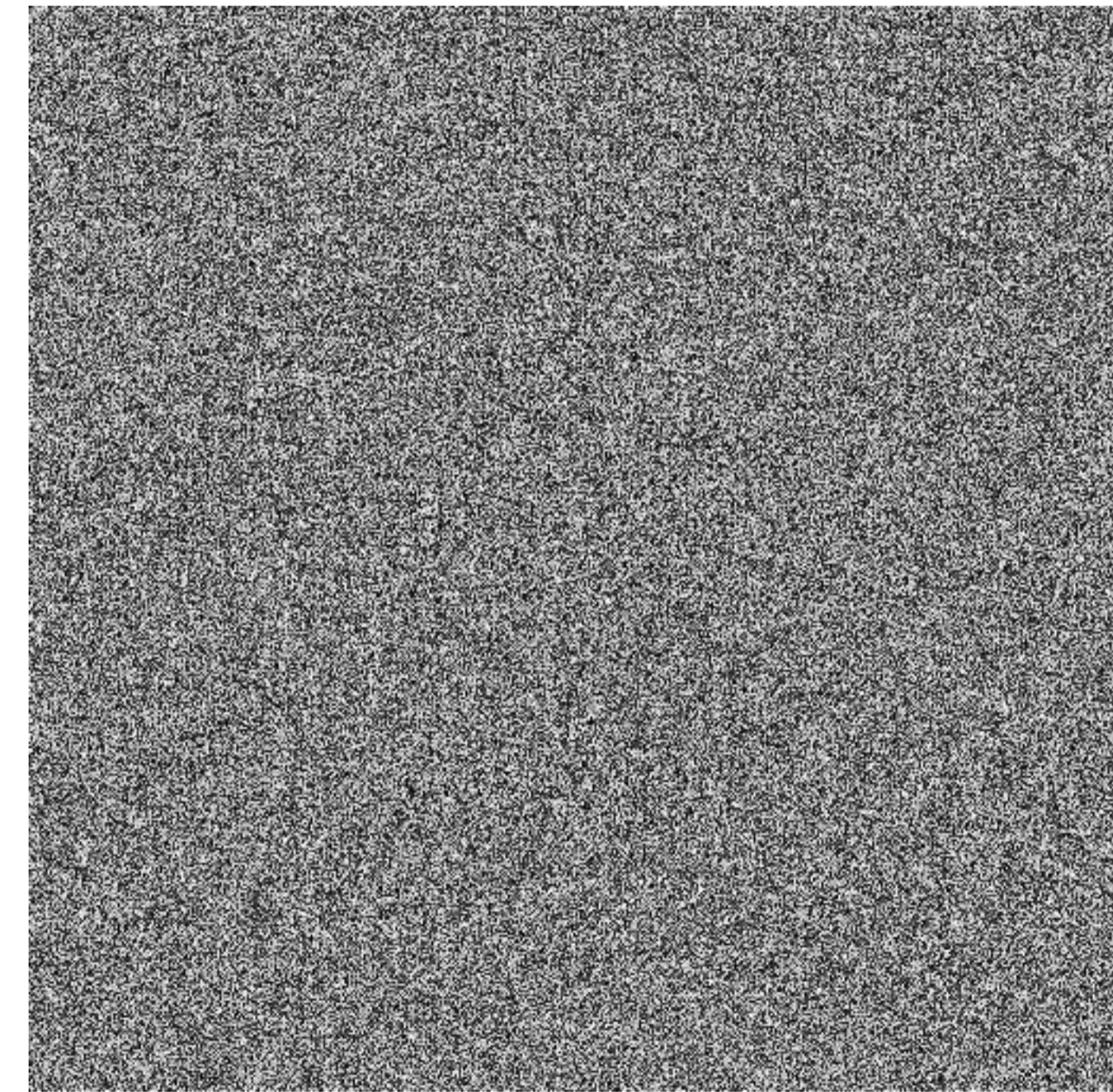
Averaged PRNU
