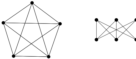
(c) K_5
