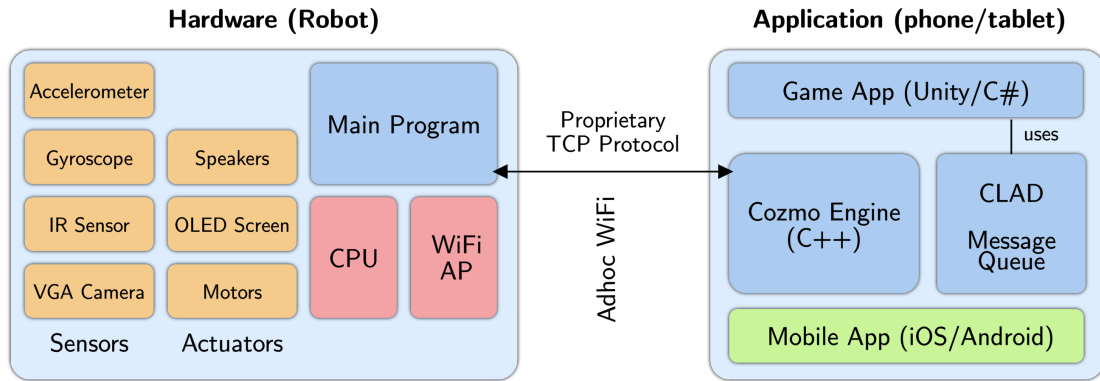
Figure 3.2. Interaction between the Robot and the mobile application stack. The main program of the robot interacts with the Cozmo Engine (C++) implemented in the mobile application through a proprietary TCP protocol established using an ad-hoc WiFi connection. [7]
