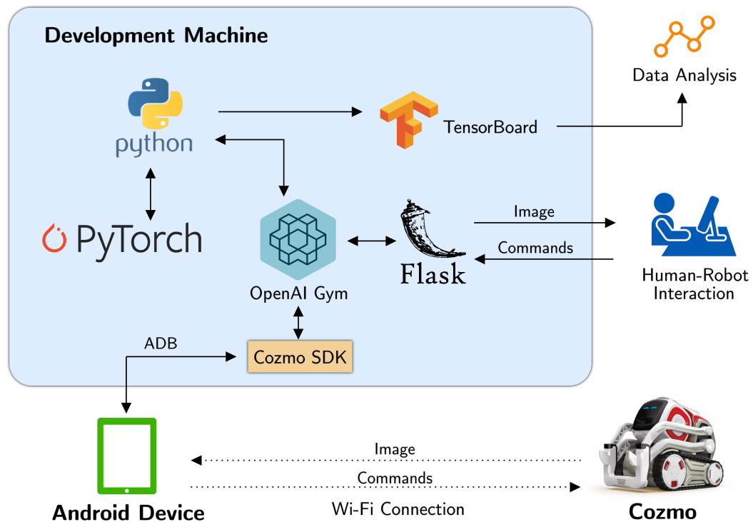
Figure 4.1. The interaction between the user and Anki Cozmo has a crucial role in this system. The main Python script utilises OpenAI Gym for the reinforcement learning component and PyTorch for the deep learning one. The user can interact with the flow of the system through a simple web app that uses OpenAI Gym and the Cozmo SDK directly to provide information for the user (e.g. images, learning information) and the robot (e.g. commands). The last component consists of TensorBoard thanks to which the script can store results that can be retrieved later by the user.
