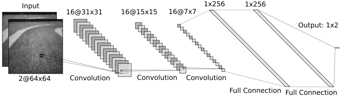
Figure 4.4. Convolutional Neural Network Architecture for Cozmo experiments. This particular example shows the model exploited as the Policy with a tensor with dimension equal to the action space size as output and two consecutive grayscale images which represents the state of the environment as input. The first part of the network consists of three convolutional layers with 16 filters of 3 \times 3 dimensions. Each level is supplemented by a batch normalisation one. The results are then flattened and concatenated with the vector of actions before entering the second part. This section consists of two fully-connected layers with 256 features. The output of this particular network represent the action to take, given the input state. This network uses ReLu as non-linearity. Before starting experiments, the network is initialised with biases equal to zero and weights set utilising Xavier initialisation [17].
