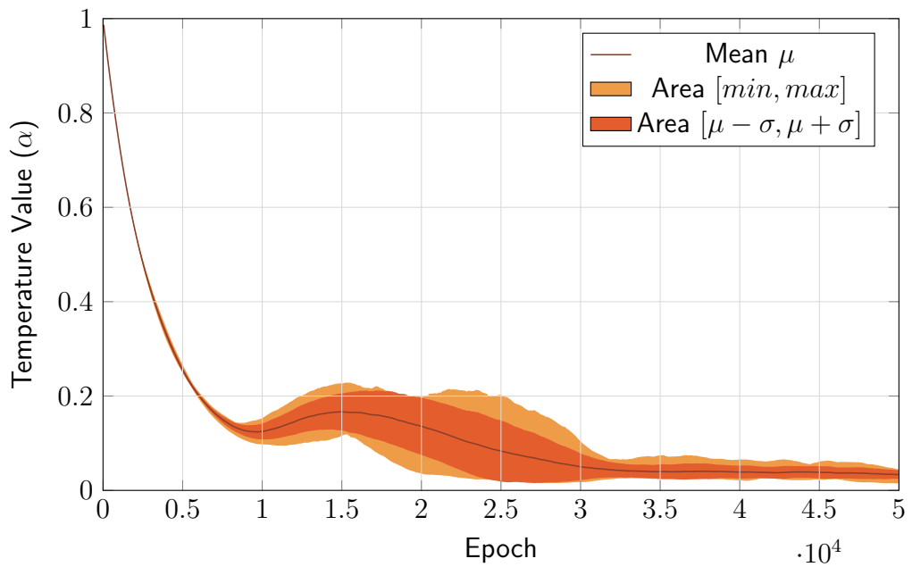
Figure 5.10. SAC Pendulum-v0 auto-tuning temperature. The graph shows the trend of the temperature parameter learned through the auto-tune process proposed by SAC authors.
