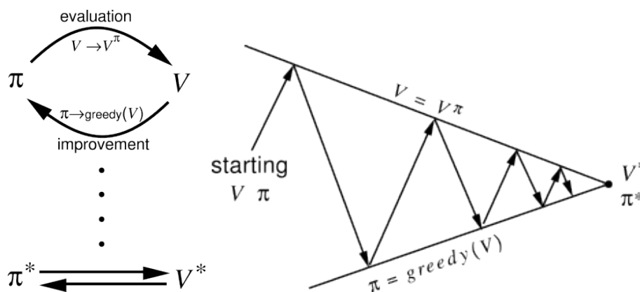
Figure 2.3. Generalised policy iteration (GPI) schema [66]. Value and policy functions compete and cooperate to reach the joint solution: the optimal value function and an optimal policy.
