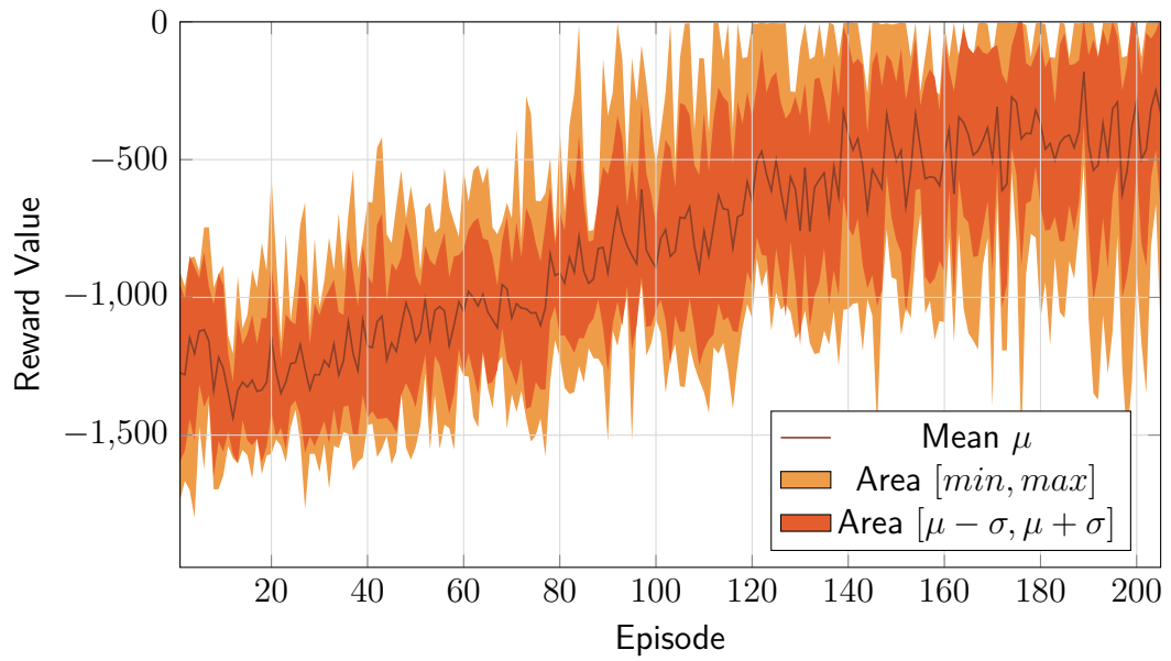
Figure 5.3. DDPG Pendulum-v0 Reward Plot. The graph reports mean, standard deviation range and min-max range of the reward of each episode over 10 runs with different seeds.
