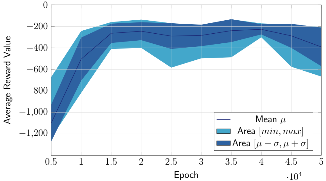
Figure 5.6. SAC Pendulum-v0 Test Average Reward Plot. The graph reports mean, standard deviation range and min-max range of the average reward obtained from 10 test episodes every 5000 epochs. They are calculated on 10 runs with different seeds.
