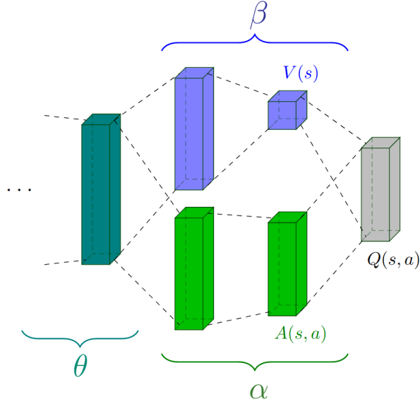
Figure 2.8. Dueling DQN architecture [73]: it consists in two stream to estimate state-value parametrised with \beta and advantages values parametrised with \alpha for each action. The last layer represent the combination of these two types of values to obtain the Q-function. [15]
