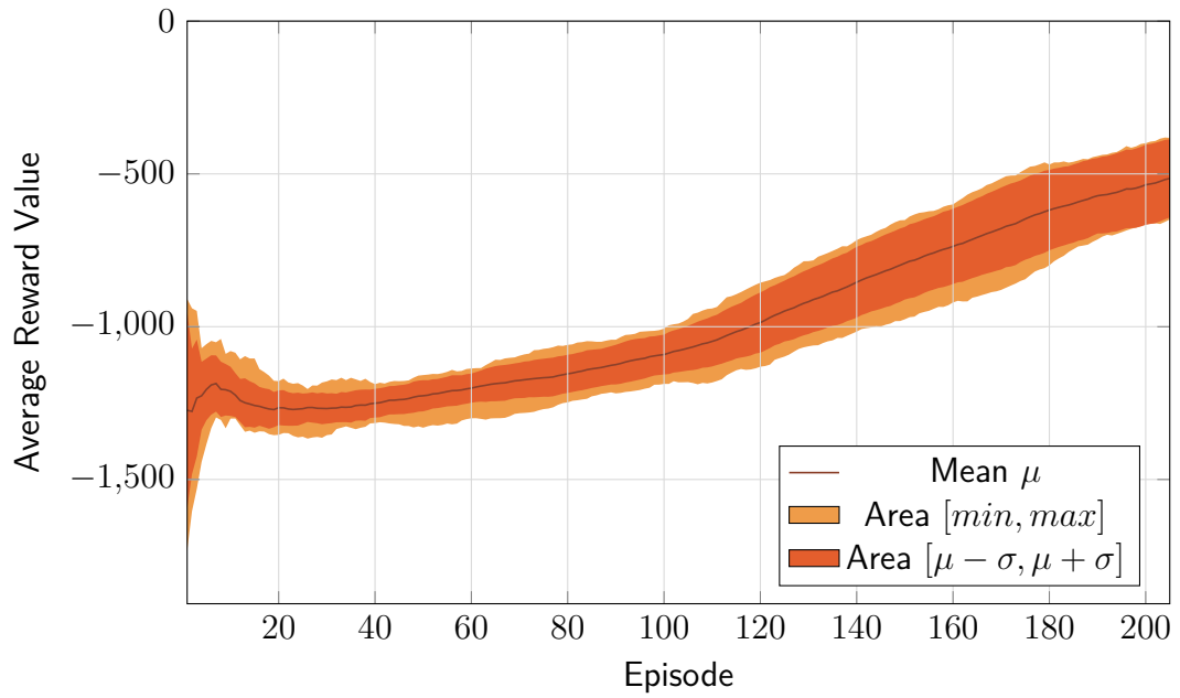
Figure 5.7. DDPG Pendulum-v0 Last 100 Episode Average Reward Plot. The graph reports mean, standard deviation range and min-max range of the last 100 episode average reward for each episode over 10 runs with different seeds.
