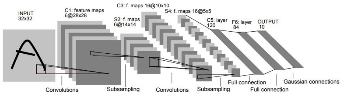
Figure 2.6. LeNet Architecture Representation. It consists of two distinct parts. The first one is composed of two stacks of convolutional and pooling layer. The last part is composed of two fully connected layers that produce the output. It represents the first compelling evidence showing the results of training convolutional neural networks by backpropagation. It was adopted to recognise digits for processing deposits in ATMs. [40]
