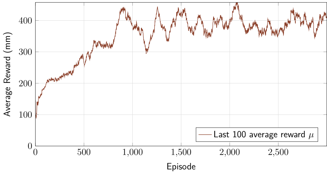
Figure 5.13. SAC CozmoDriver-v0 Last 100 Episode Average Reward Plot. The graph reports the last 100 episode average reward for each episode.
