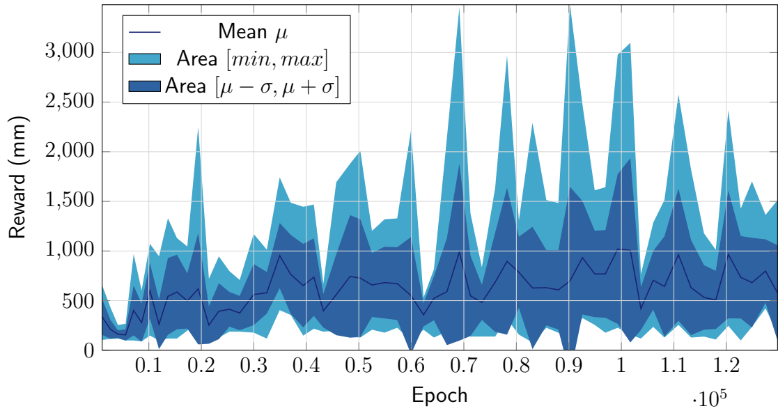
Figure 5.14. SAC CozmoDriver-v0 Test Reward Plot. The graph reports mean, standard deviation range and min-max range of the average reward obtained from 10 test episodes every 50 episodes.
