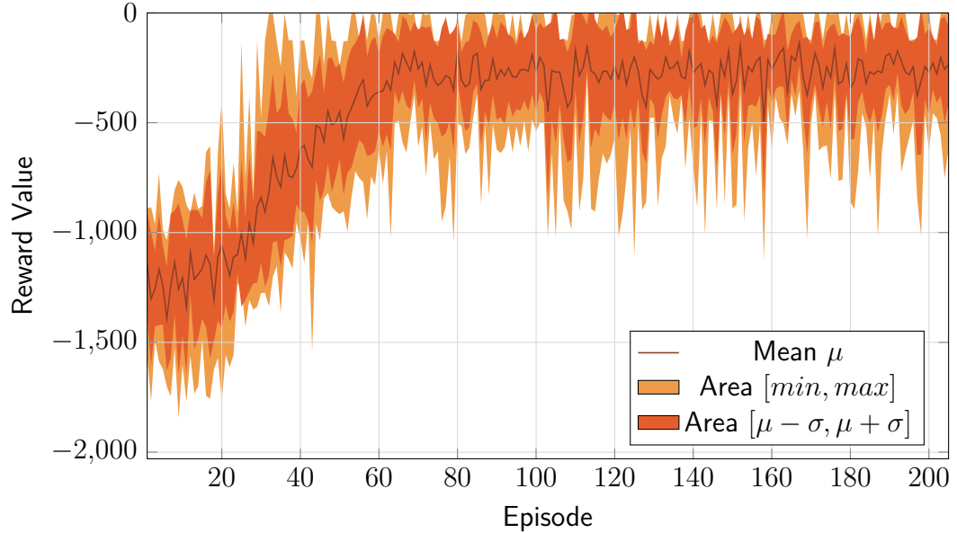
Figure 5.4. SAC Pendulum-v0 Reward Plot. The graph reports mean, standard deviation range and min-max range of the reward of each episode over 10 runs with different seeds.
