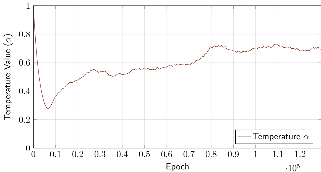
Figure 5.11. SAC CozmoDriver-v0 auto-tuned temperature. The graph shows the trend of the temperature parameter learned through the auto-tune process proposed by SAC authors.
