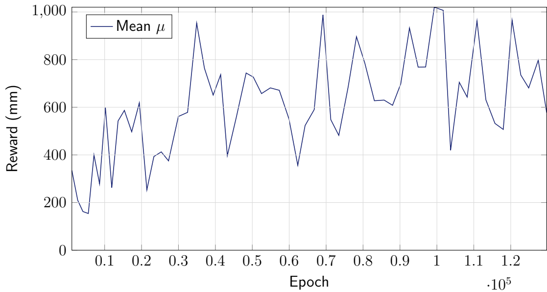
Figure 5.15. SAC CozmoDriver-v0 Test Average Reward Plot. The graph reports with a focus on the average reward obtained from 10 test episodes every 50 episodes.
