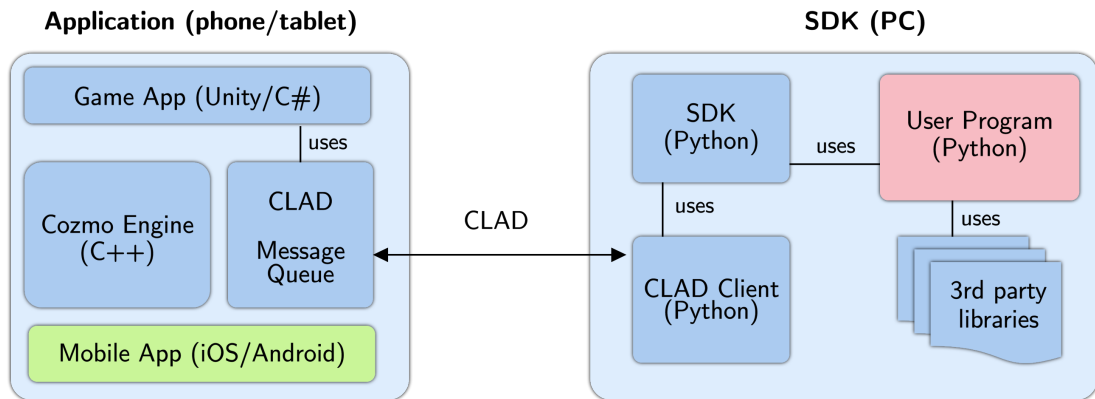
Figure 3.3. Interaction between the mobile application stack and the Python user program. Anki designed a C-like Abstract Data Language (CLAD) to implement the connection between the Cozmo SDK and the Cozmo Engine on the mobile application. This approach puts a decoupling layer between Python interfaces and low-level functions to make prototyping easier and fast-forwarding for developers. [7]
