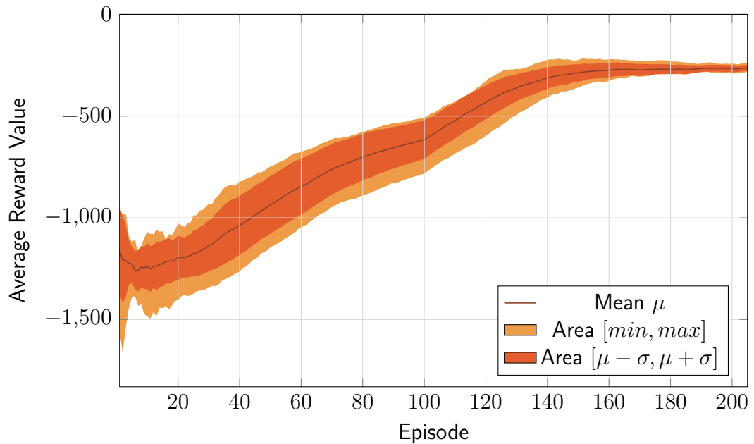
Figure 5.8. SAC Pendulum-v0 Last 100 Episode Average Reward Plot. The graph reports mean, standard deviation range and min-max range of the last 100 episode average reward for each episode over 10 runs with different seeds.
