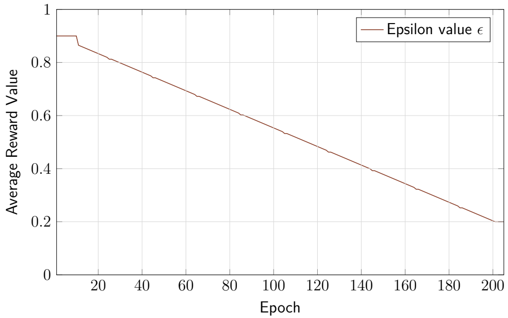
Figure 5.9. DDPG Pendulum-v0 Noise Epsilon Decay. The graph shows the trend of the noise epsilon decay applied to the Ornstein Uhlenbeck noise in DDPG.
