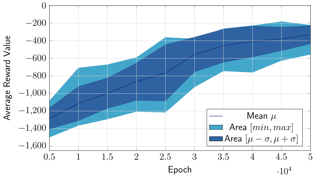
Figure 5.5. DDPG Pendulum-v0 Test Average Reward Plot. The graph reports mean, standard deviation range and min-max range of the average reward obtained from 10 test episodes every 5000 epochs. They are calculated on 10 runs with different seeds.
