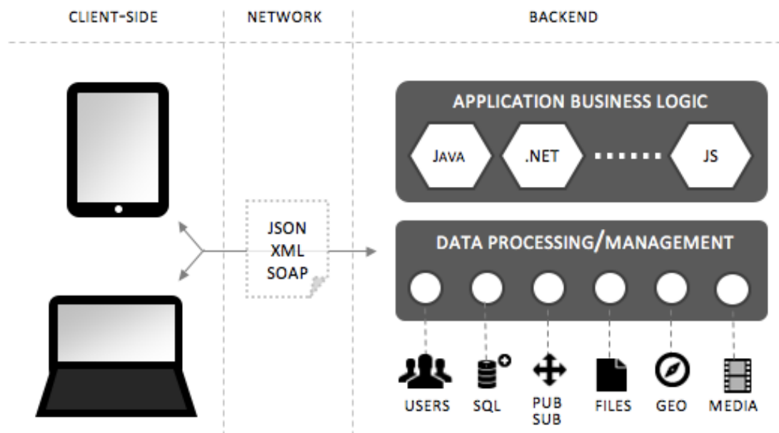
图 33: Backend As A Service
