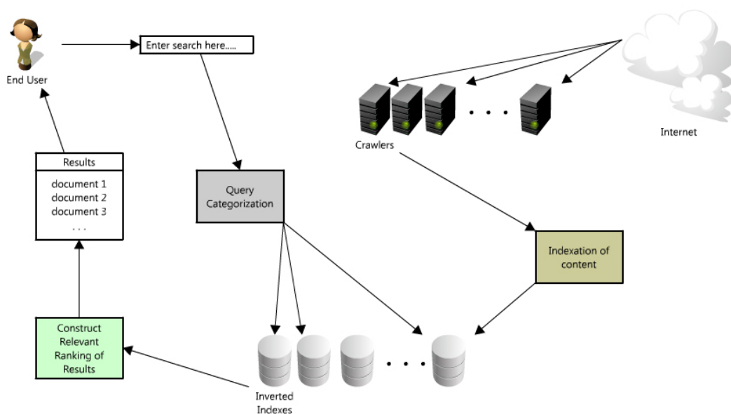
图 77: search-engine-arch
