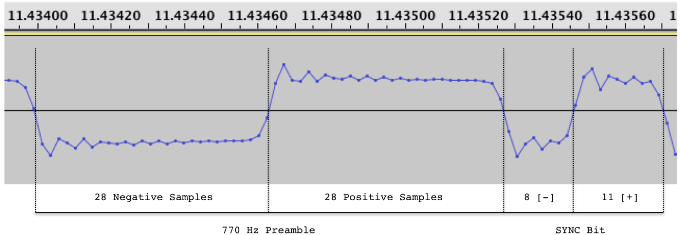
Figure 2 illustrates the end of the 770 Hz preamble and the SYNC Bit, zoomed to expose the digital data. The lines that connect the dots are simply that, lines, and they do not represent data.
