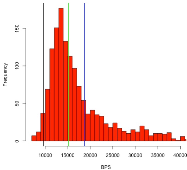
Figures 6: Histogram of the effective BPS of 1469 virtualapple.org disk images. The blue line is the mean (average), the green line is the median (halfway mark), and the black line is 9600 BPS.
