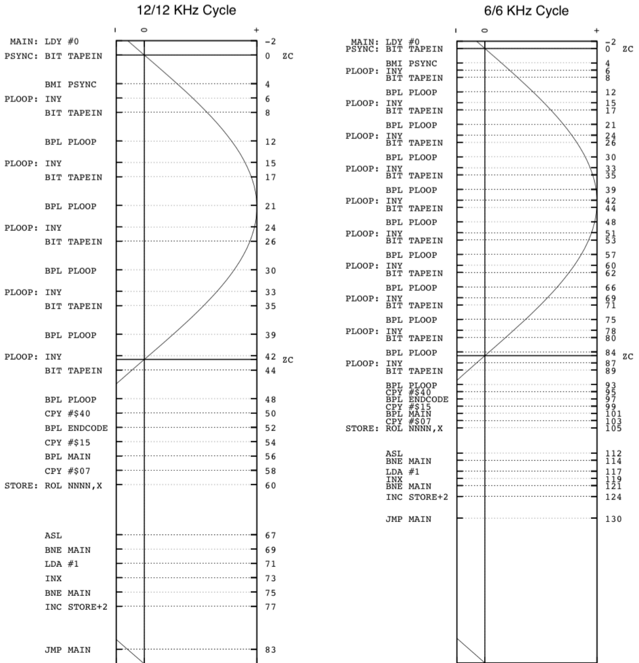
Figure 3 superimposes the c2t Apple II instructions on normalized waveforms that represent 12000 Hz and 6000 Hz full cycles respectively. On the left y-axis are the Apple II instructions. On the right y-axis is the accumulated Apple II clock cycle count (ticks). ZC represents the zero crossing.
