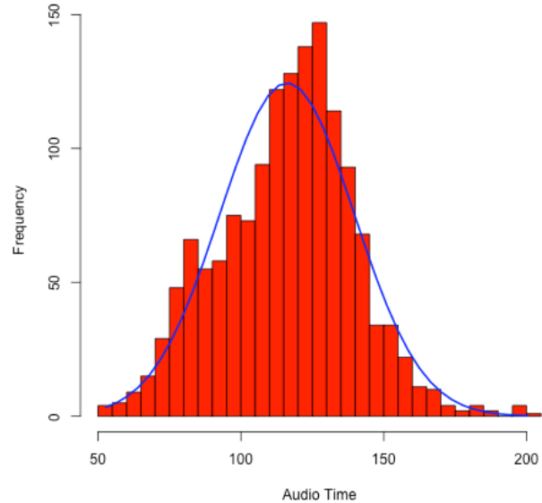
Figure 7: Histogram of the no-format total audio time in seconds of 1469 virtualapple.org disk images.
