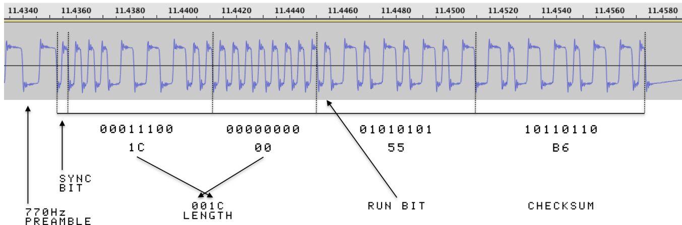
Figure 1 illustrates the header for a small FP BASIC program that I captured using the BASIC SAVE command. What you do not see left of the SYNC Bit is 10 seconds of 770 Hz tone and about 1.4 seconds of nothing (first had to press record on my recorder and then type "SAVE" and press RETURN-- that took about 1.4 seconds). Each bit is represented by a full cycle square wave. Narrow bits (the zeroes) have higher frequencies (2000 Hz) and wider bits (the ones) have lower frequencies (1000 Hz).
