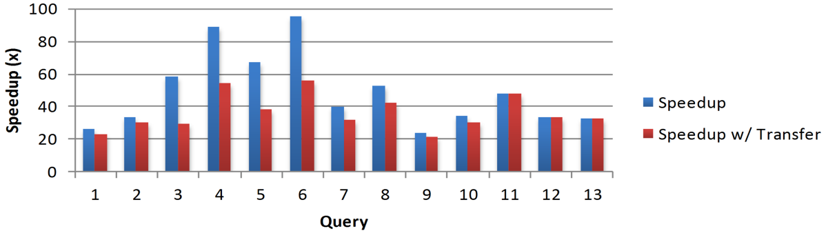
Figure 1: The speedup of query execution on the GPU for each of the 13 queries considered, both including and excluding the results transfer time
