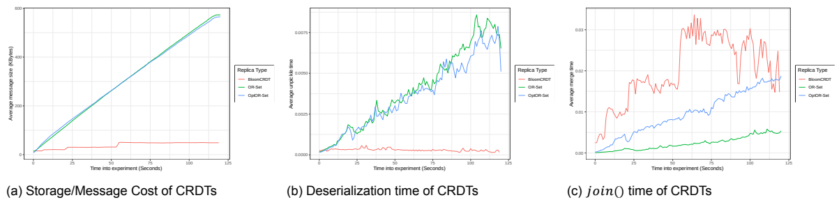
Figure 5.2: Experiment comparing BloomCRDT, OR-Set and OptOR-Set with network churn
