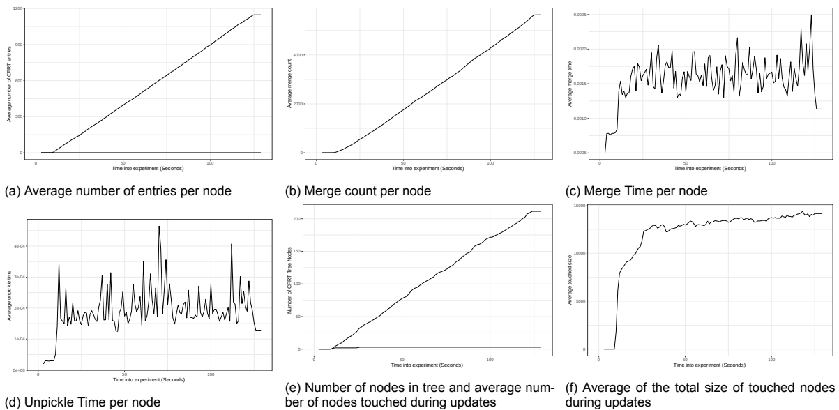
Figure 5.3: Demonstrating \log() scaling of CFRT
