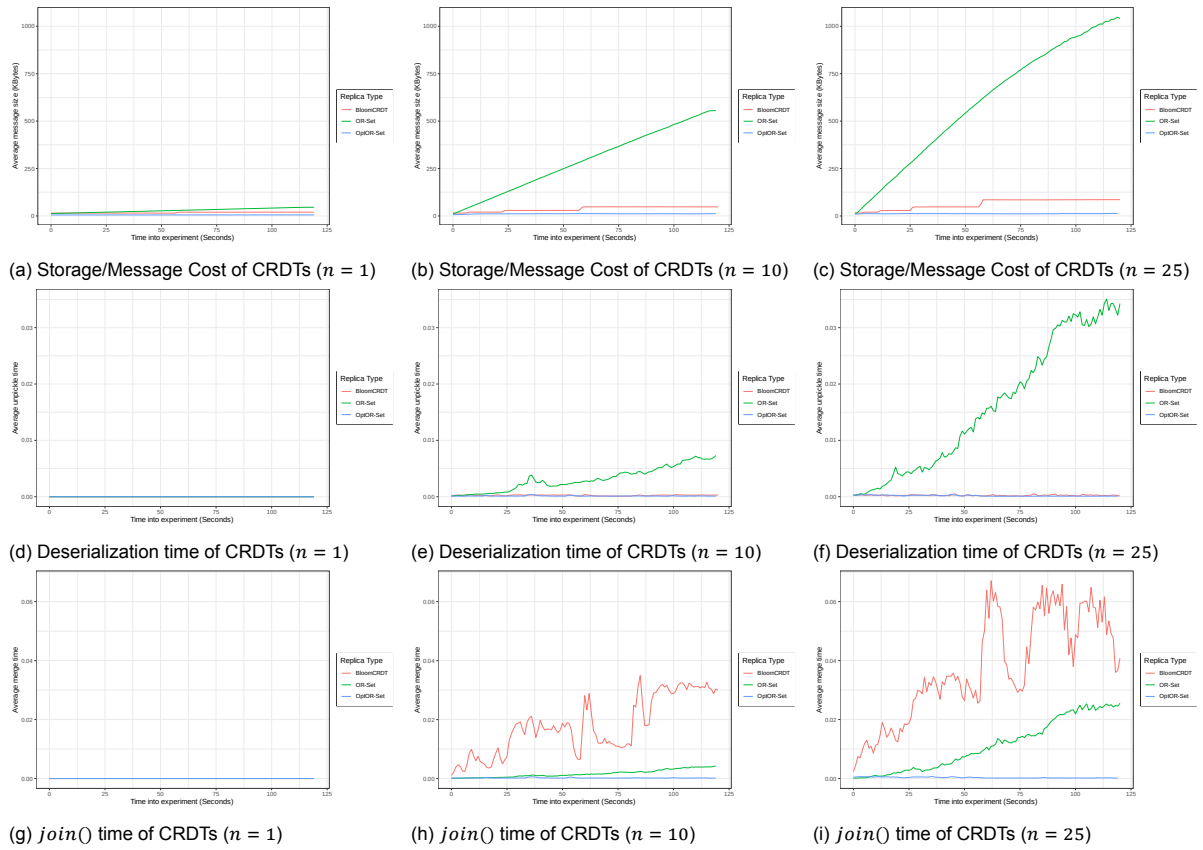
Figure 5.1: Experiment comparing BloomCRDT, OR-Set and OptOR-Set
