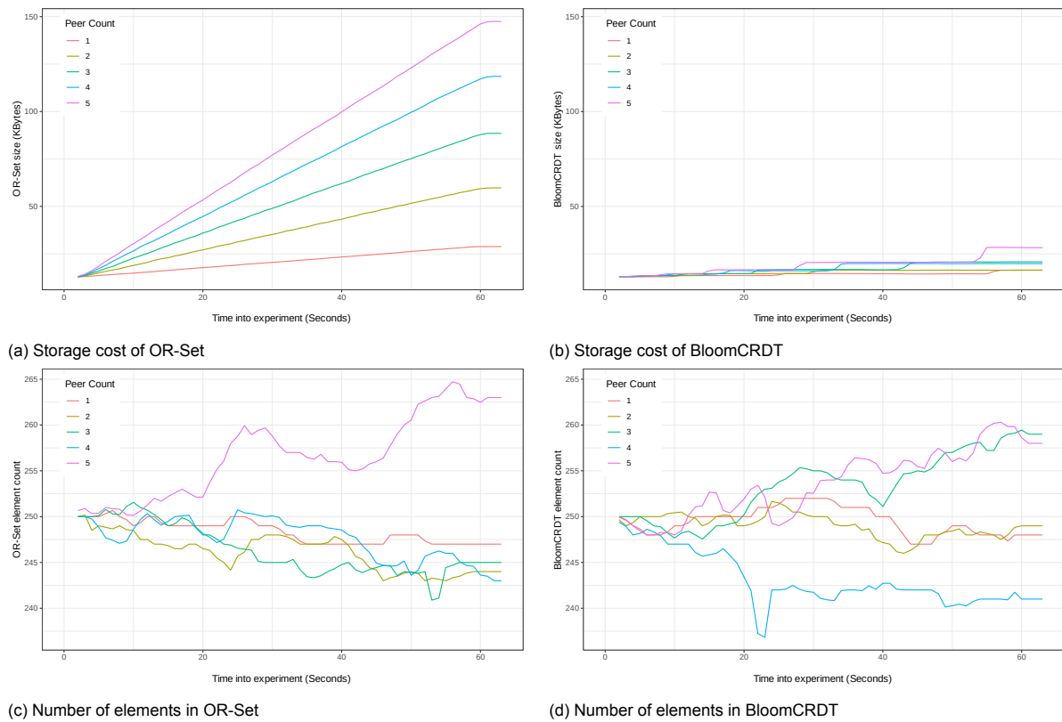
Figure 5.1: Experiment comparing BloomCRDT to OR-Set
