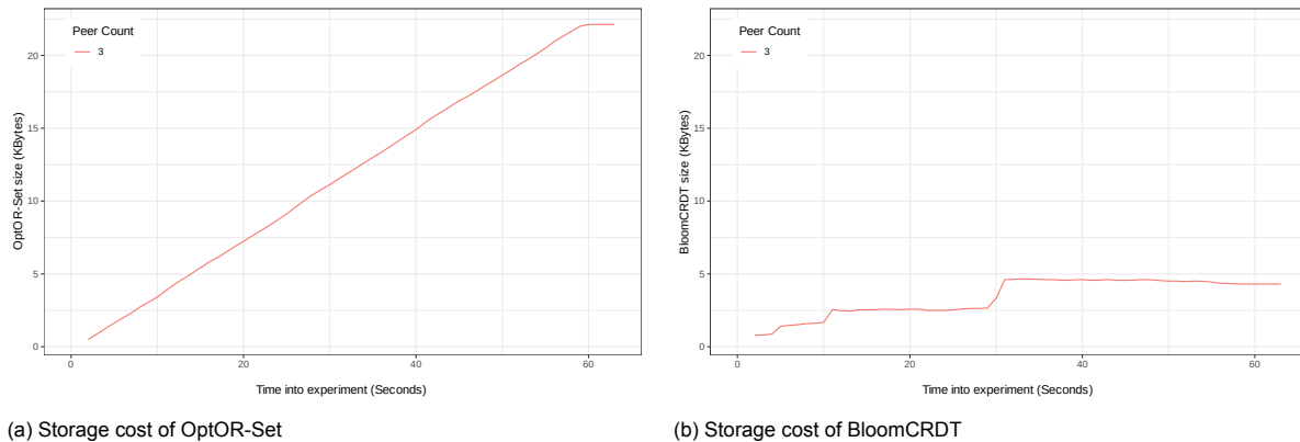
Figure 5.2: Experiment comparing BloomCRDT to OptOR-Set with network churn
