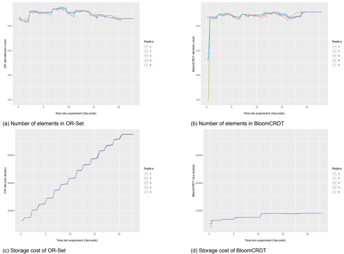
Figure 5.1: Experiment comparing BloomCRDT to OR-Set
