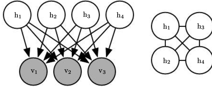
Figure 19.2: The graph structure of a binary sparse coding model with four hidden units. ( Left ) The graph structure of p(\mathbf{h}, \mathbf{v}) . Note that the edges are directed, and that every two hidden units are co-parents of every visible unit. ( Right ) The graph structure of p(\mathbf{h} | \mathbf{v}) . In order to account for the active paths between co-parents, the posterior distribution needs an edge between all of the hidden units.
