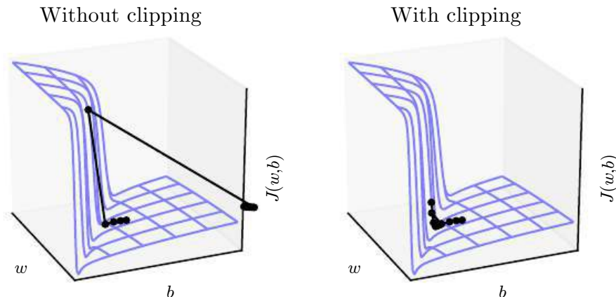
Figure 10.17: Example of the effect of gradient clipping in a recurrent network with two parameters \mathbf{w} and \mathbf{b} . Gradient clipping can make gradient descent perform more reasonably in the vicinity of extremely steep cliffs. These steep cliffs commonly occur in recurrent networks near where a recurrent network behaves approximately linearly. The cliff is exponentially steep in the number of time steps because the weight matrix is multiplied by itself once for each time step. ( Left ) Gradient descent without gradient clipping overshoots the bottom of this small ravine, then receives a very large gradient from the cliff face. The large gradient catastrophically propels the parameters outside the axes of the plot. ( Right ) Gradient descent with gradient clipping has a more moderate reaction to the cliff. While it does ascend the cliff face, the step size is restricted so that it cannot be propelled away from steep region near the solution. Figure adapted with permission from Pascanu et al. (2013a) .
