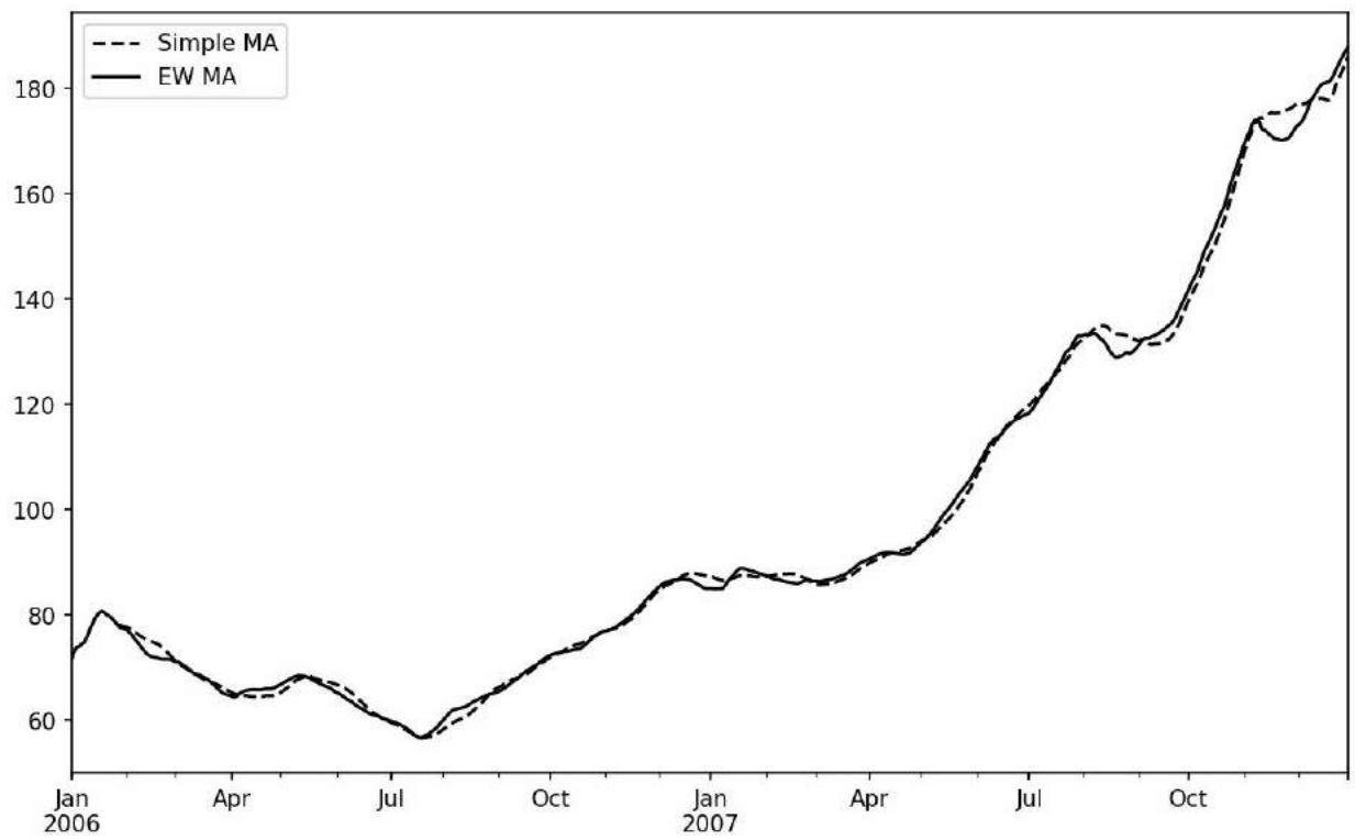
Figure 11-7. Simple moving average versus exponentially weighted
