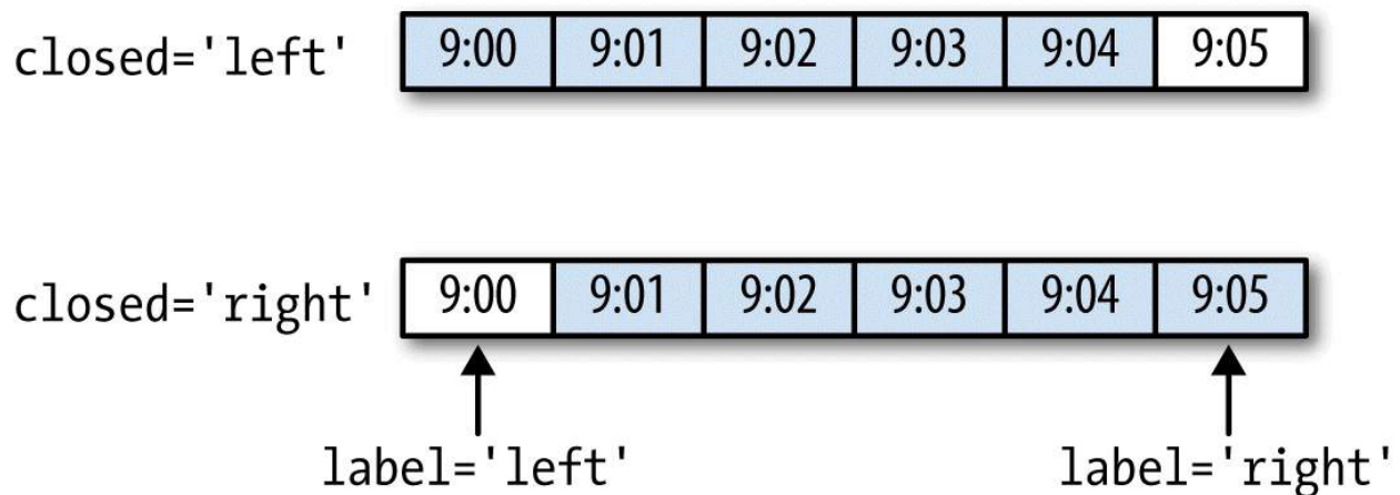
Figure 11-3. Five-minute resampling illustration of closed, label conventions
