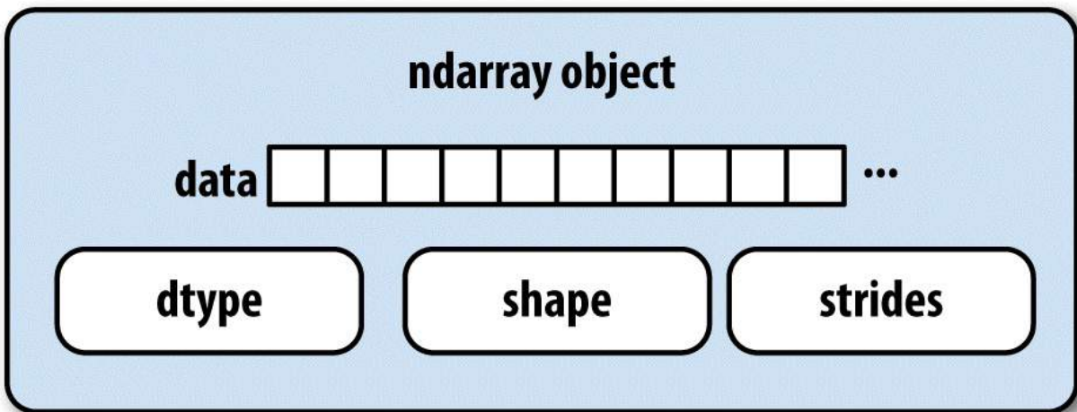
Figure A-1. The NumPy ndarray object
