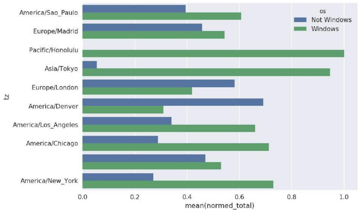
Figure 14-3. Percentage Windows and non-Windows users in top-occurring time zones
