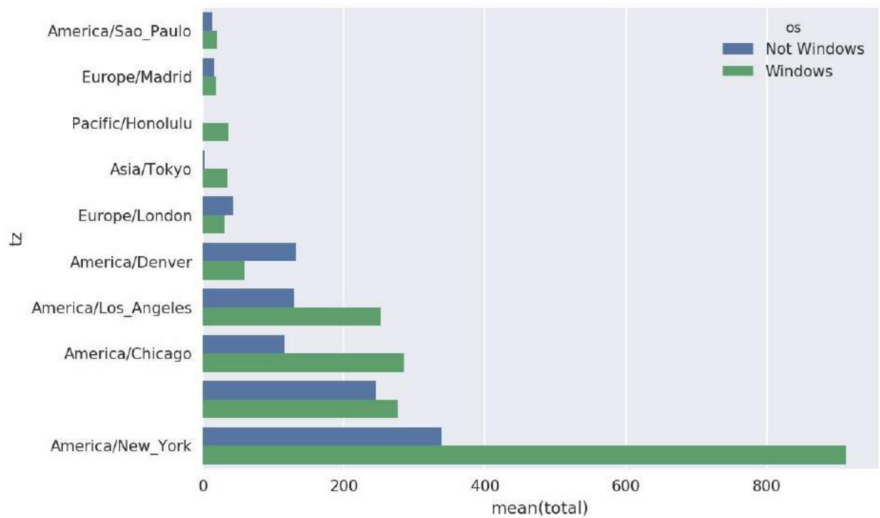
Figure 14-2. Top time zones by Windows and non-Windows users
