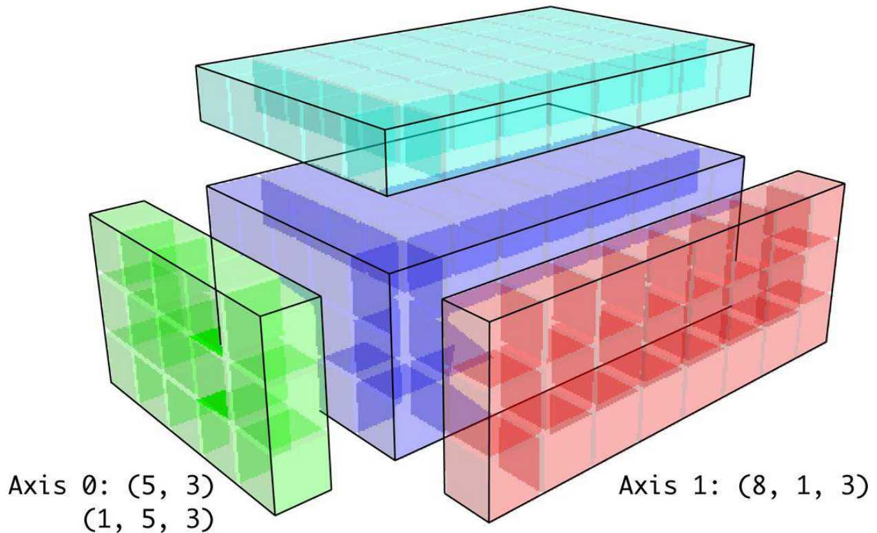
Figure A-7. Compatible 2D array shapes for broadcasting over a 3D array
