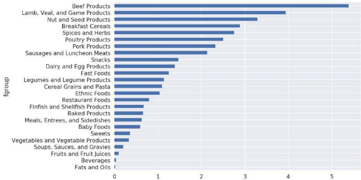
Figure 14-11. Median zinc values by nutrient group
