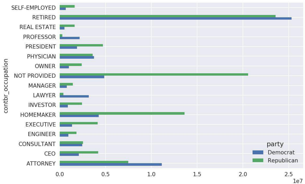
Figure 14-12. Total donations by party for top occupations
