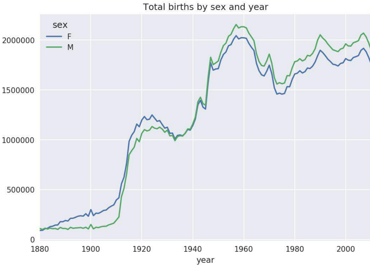
Figure 14-4. Total births by sex and year
