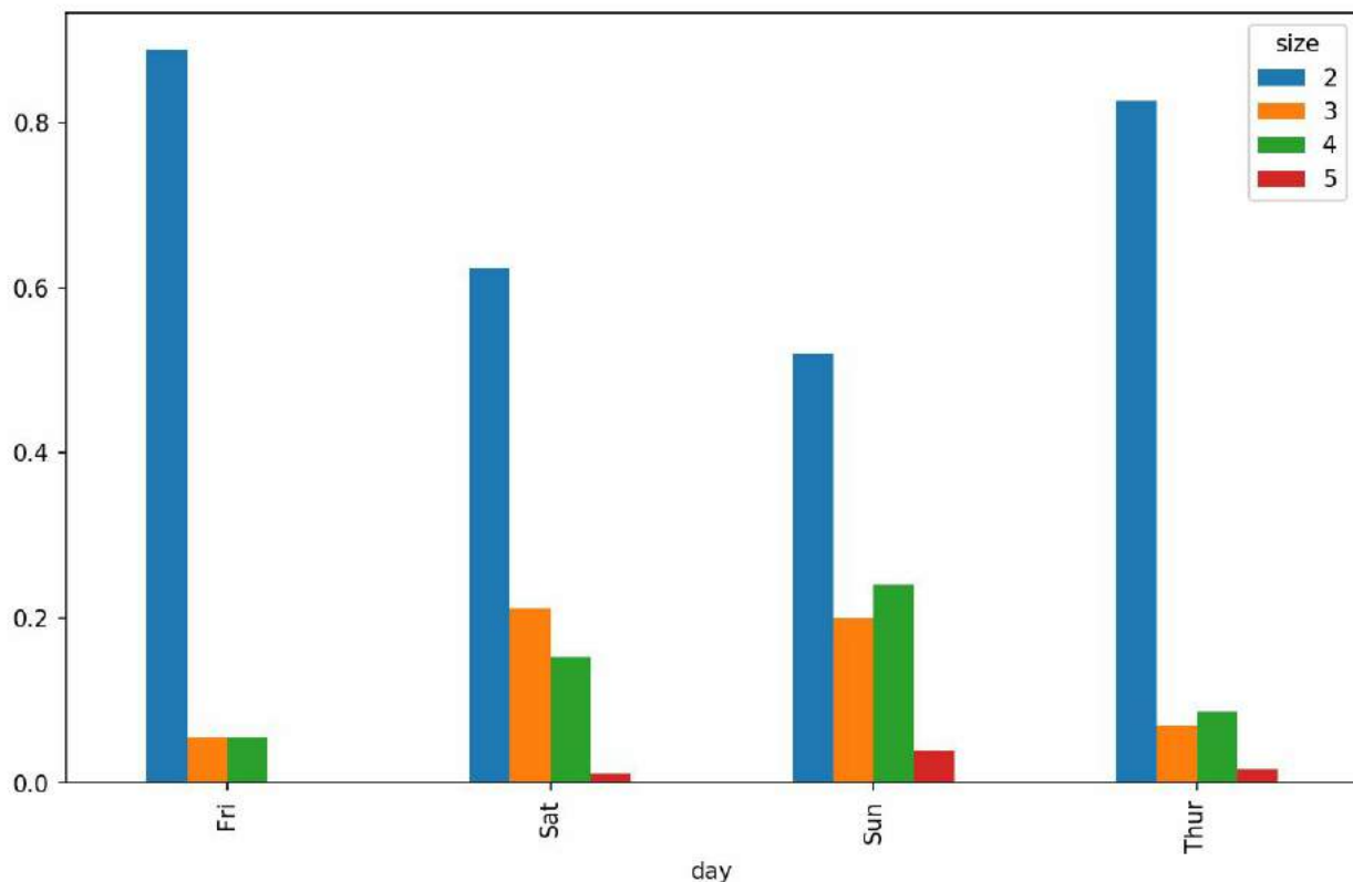
Figure 9-18. Fraction of parties by size on each day
