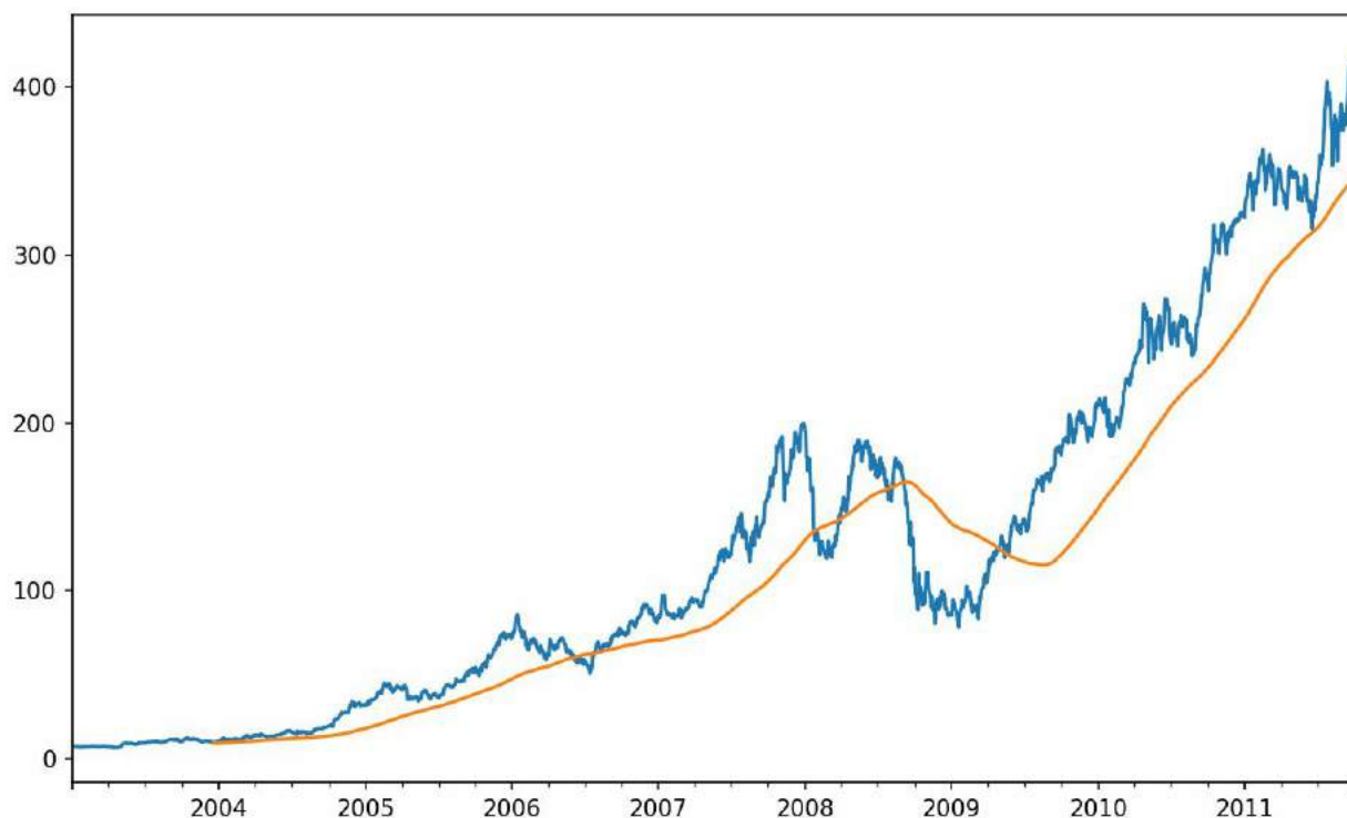
Figure 11-4. Apple Price with 250-day MA
