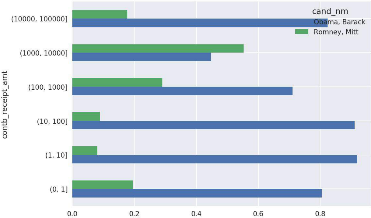
Figure 14-13. Percentage of total donations received by candidates for each donation size
