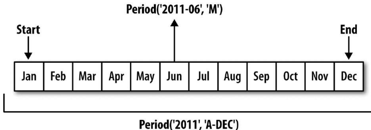
Figure 11-1. Period frequency conversion illustration
