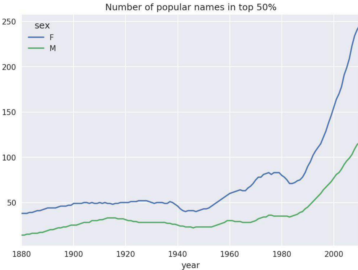
Figure 14-7. Plot of diversity metric by year
