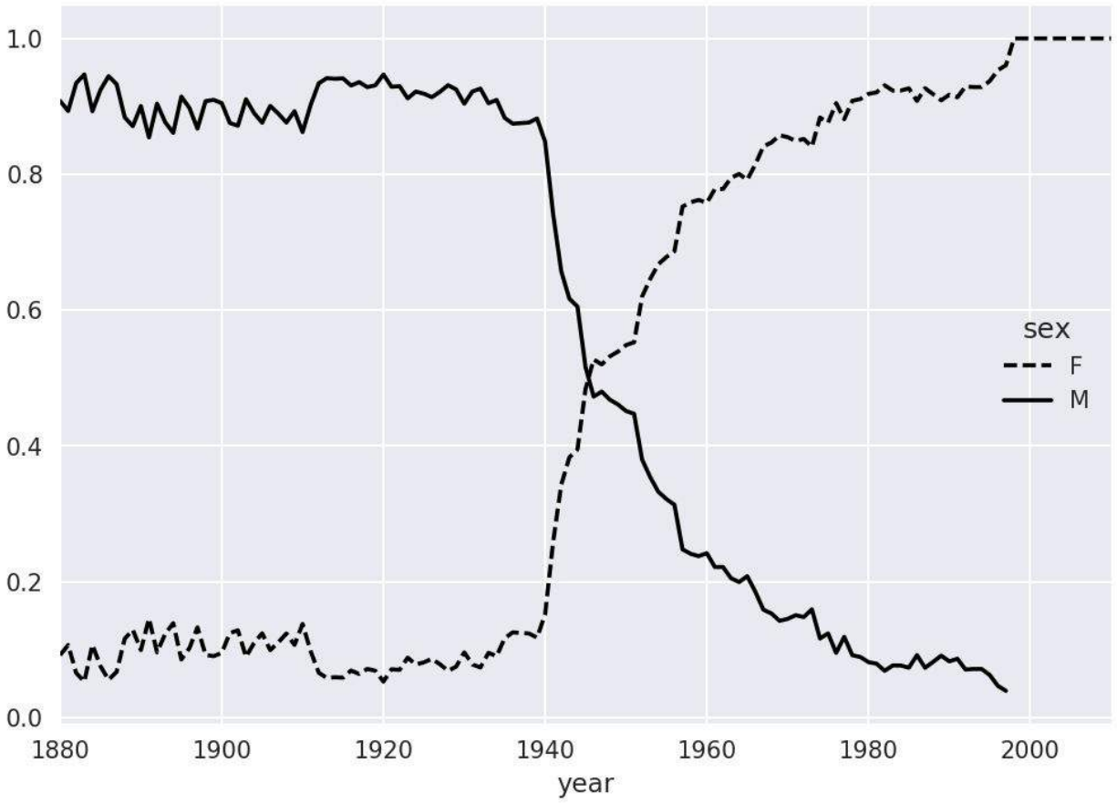
Figure 14-10. Proportion of male/female Lesley-like names over time
