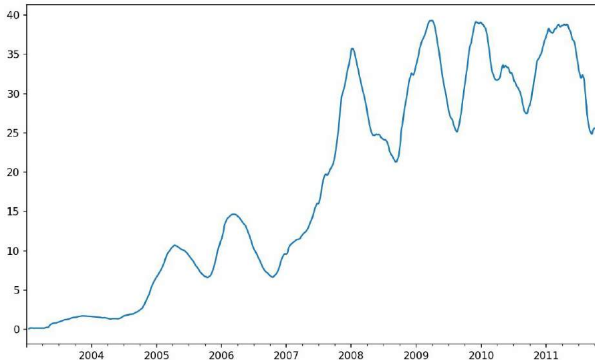
Figure 11-5. Apple 250-day daily return standard deviation
