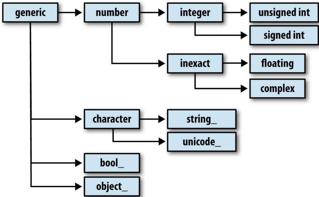
Figure A-2. The NumPy dtype class hierarchy
