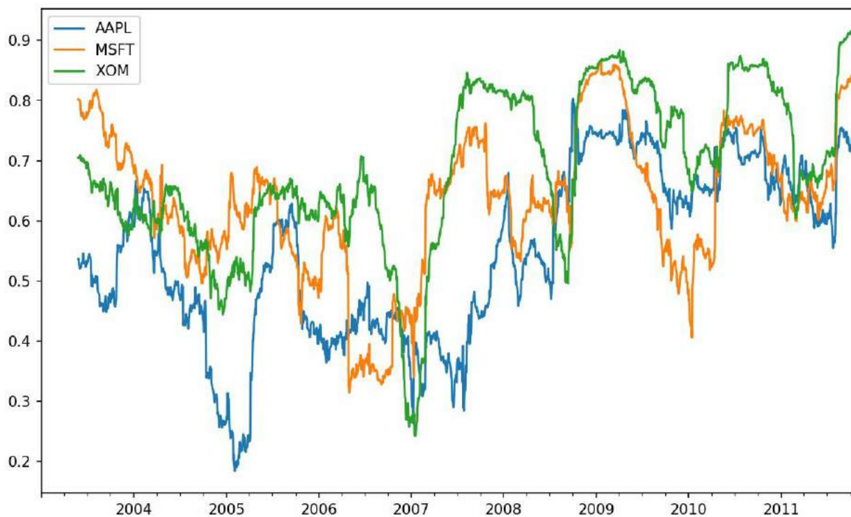
Figure 11-9. Six-month return correlations to S&P 500
