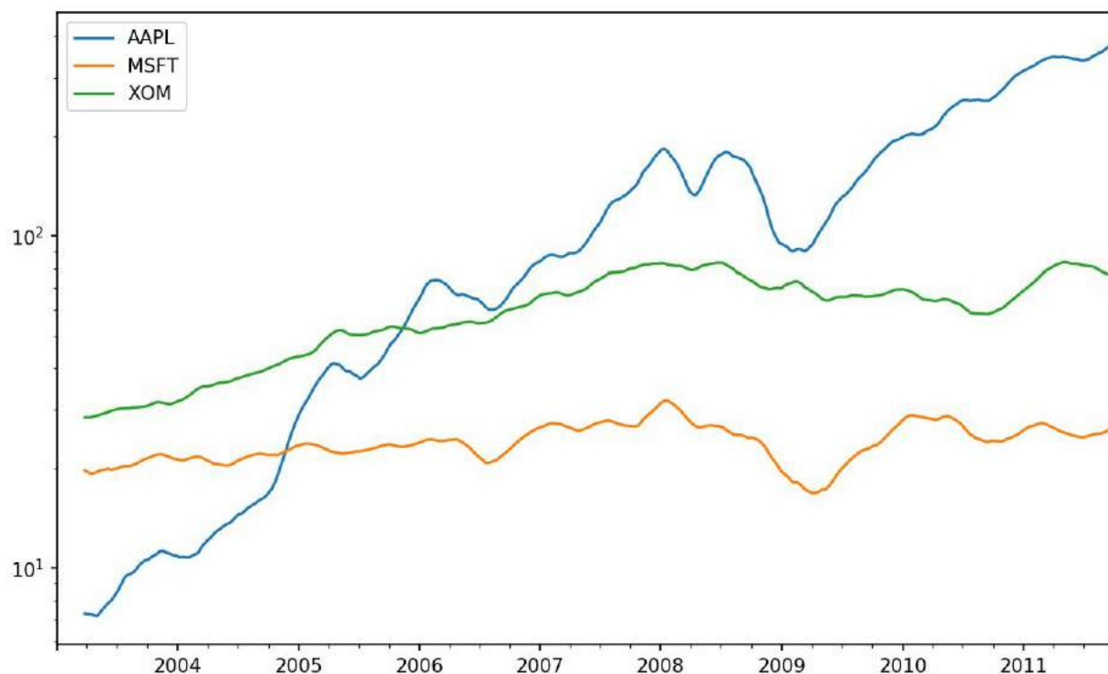
Figure 11-6. Stocks prices 60-day MA (log Y-axis)
