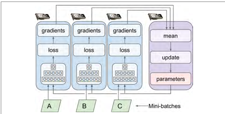
Figure 12-17. Data parallelism
