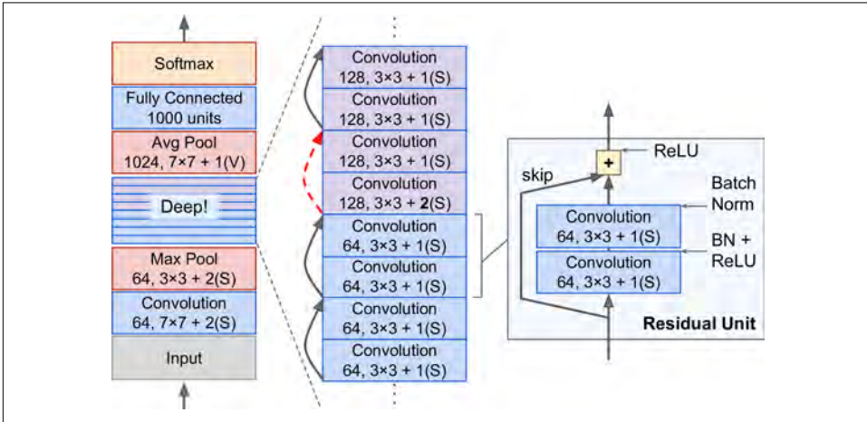
Figure 13-14. ResNet architecture
