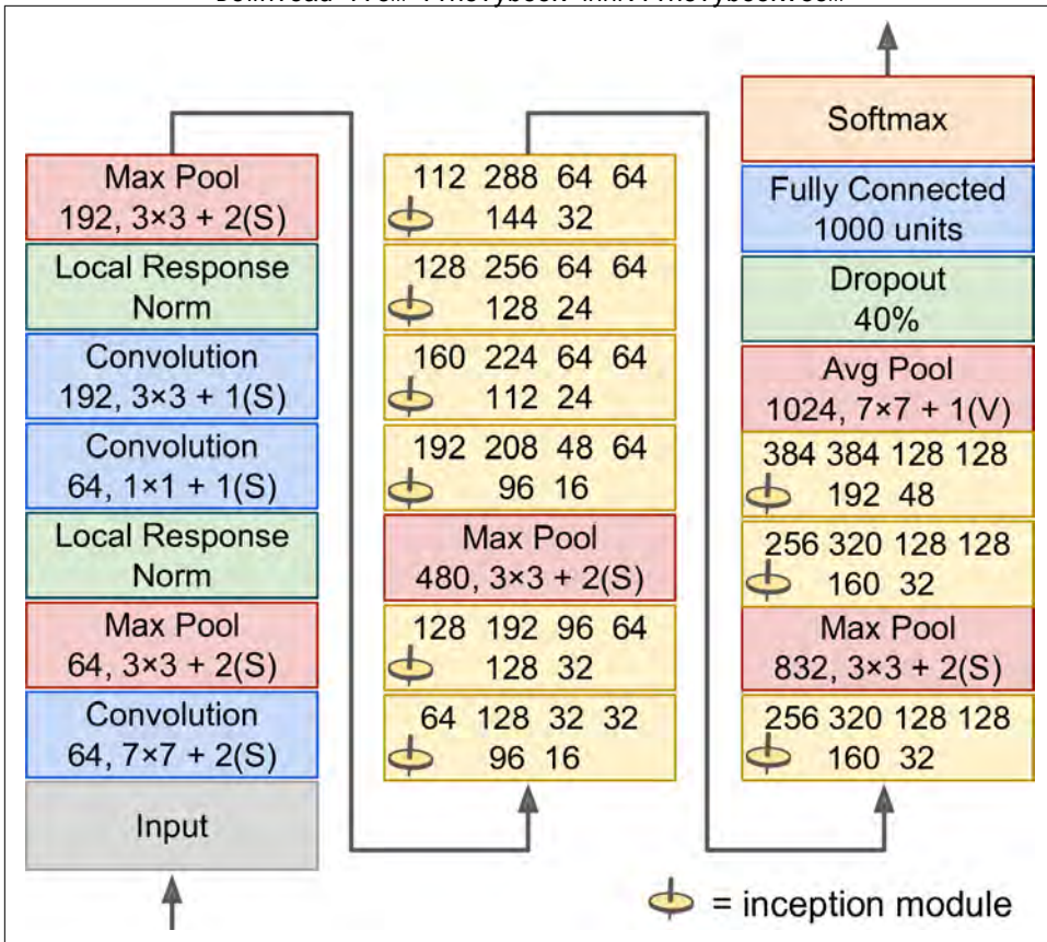
Figure 13-11. GoogLeNet architecture
