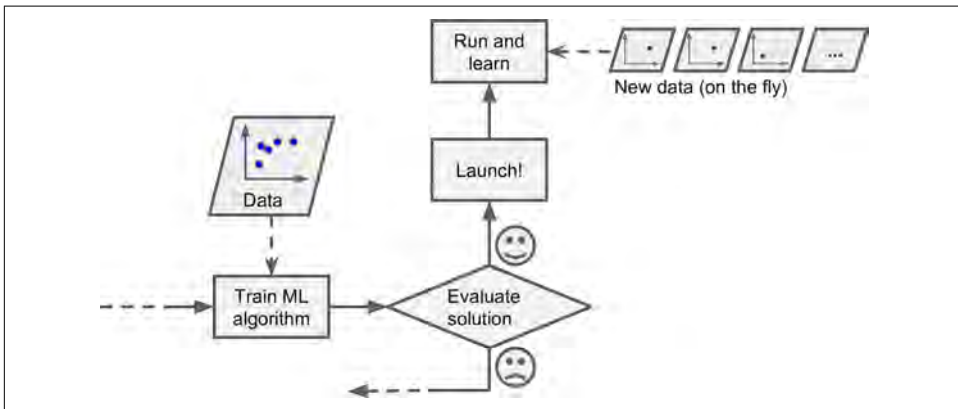
Figure 1-13. Online learning
