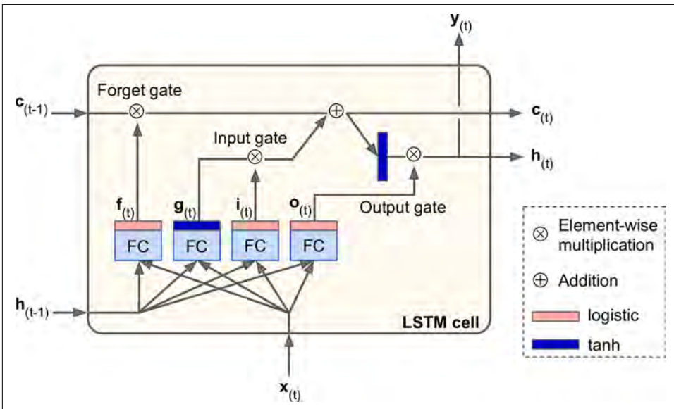
Figure 14-13. LSTM cell
