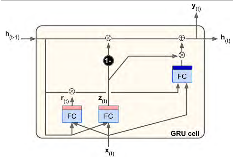
Figure 14-14. GRU cell
