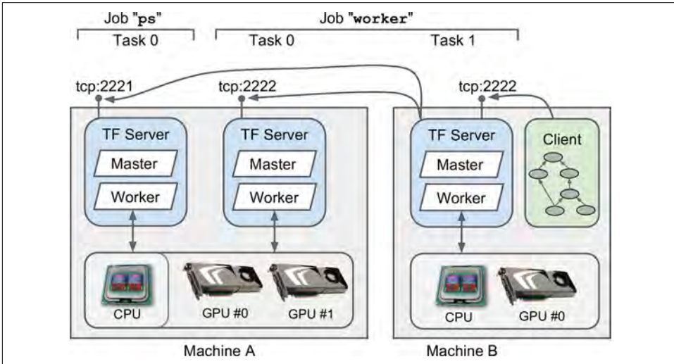
Figure 12-6. TensorFlow cluster
