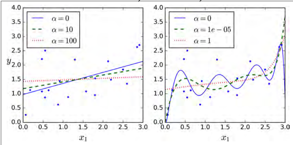
Figure 4-17. Ridge Regression
