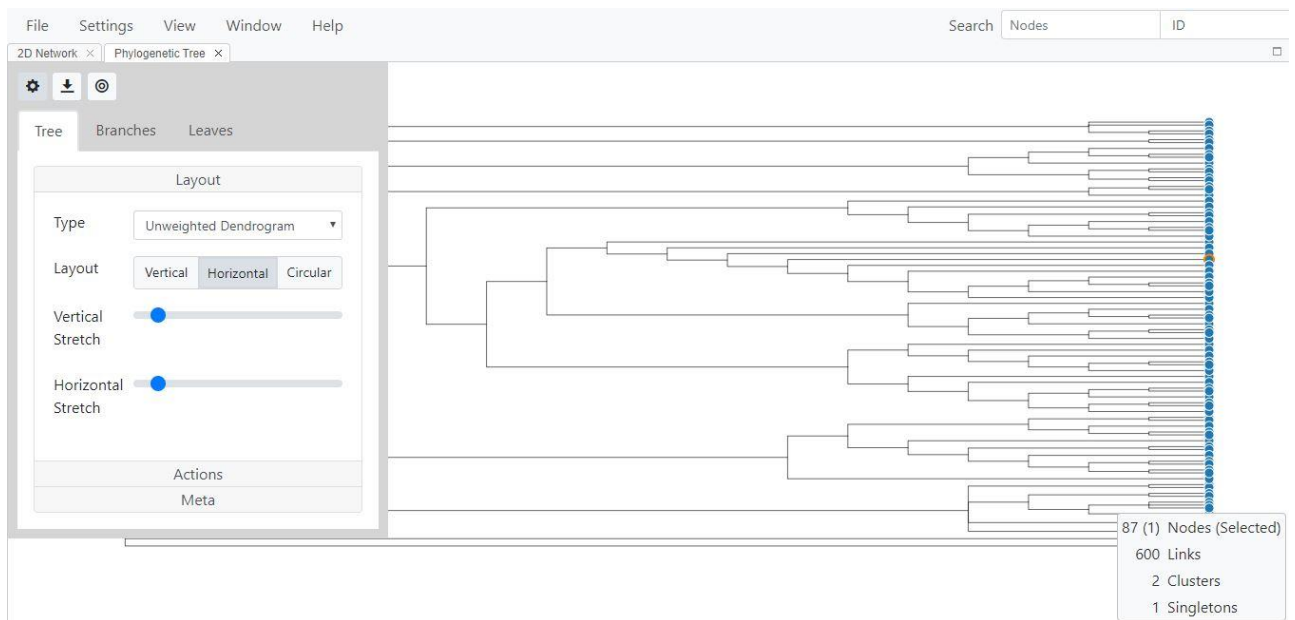
Fig. 104. Unweighted dendrogram
