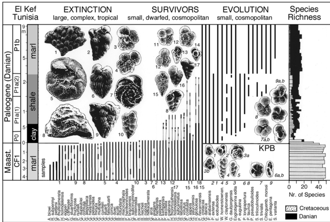
Fig. 4. KP extinction pattern at El Kef, Tunisia, shows all large tropical to subtropical species extinct or near the KP (2/3 of all species, SEM illustrations 1–10, numbers keyed to species), the short-term survivorship of small ecologically more tolerant species (1/3 of the species, SEMs 11–18) including a single long-term survivor ( Guembeltria cretacea , SEM 14). Early Danian evolution begins within a few thousand years of the mass extinction but diversity remains low and species small (SEM 1–9) marking high-stress conditions over ~500 ky of the earliest Danian. SEM illustrations are shown in relative species sizes in the assemblages. Faunal data updated from Keller (1988a).
