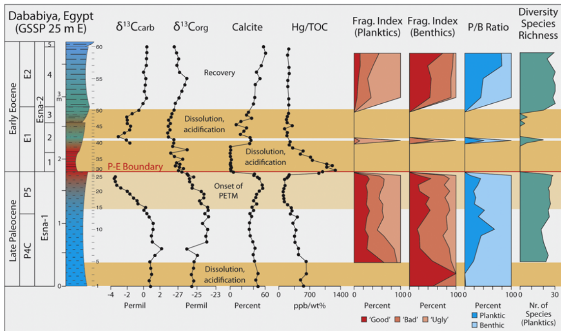
Fig. 14. Paleoenvironmental proxies for the PETM transition at Dababiya, Egypt. Dissolution first appears in zone P4C coincident with high Hg/TOC values. The onset of the PETM begins with gradually decreasing \delta^{13}\text{C} values in zone P5 that reached maximum at the PEB. Near total \text{CaCO}_3 dissolution in the lower part of zone E1 and strong dissolution in the upper part marks an interval nearly devoid of marine calcareous plankton during the PETM and signals strong ocean acidification despite the onset of recovery in \delta^{13}\text{C} and \text{CaCO}_3 . Faunal recovery begins in zone E2 with increasing \delta^{13}\text{C} values and \text{CaCO}_3 reaching 60%. Data table (Table S3) in Supplementary materials S2.
