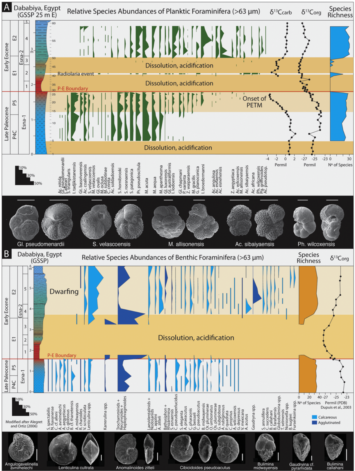
Fig. 13. (A) Relative abundances of planktic foraminifera, carbon stable isotopes and species richness at Dababiya, Egypt, 25 m east of the GSSP outcrop. The PETM interval spans from its gradual onset 75 cm below to 1 m above the PEB and is marked by near total carbonate dissolution. Another strong dissolution interval at the base of the section has common benthic species but only rare planktics. Faunal data from this study, isotope data from Khozyem et al. (2014, 2015). (B) Relative abundances of benthic foraminifera show a major faunal turnover but few species extinctions (18%, 7 species). Faunal data from Alegret and Ortiz (2006).
