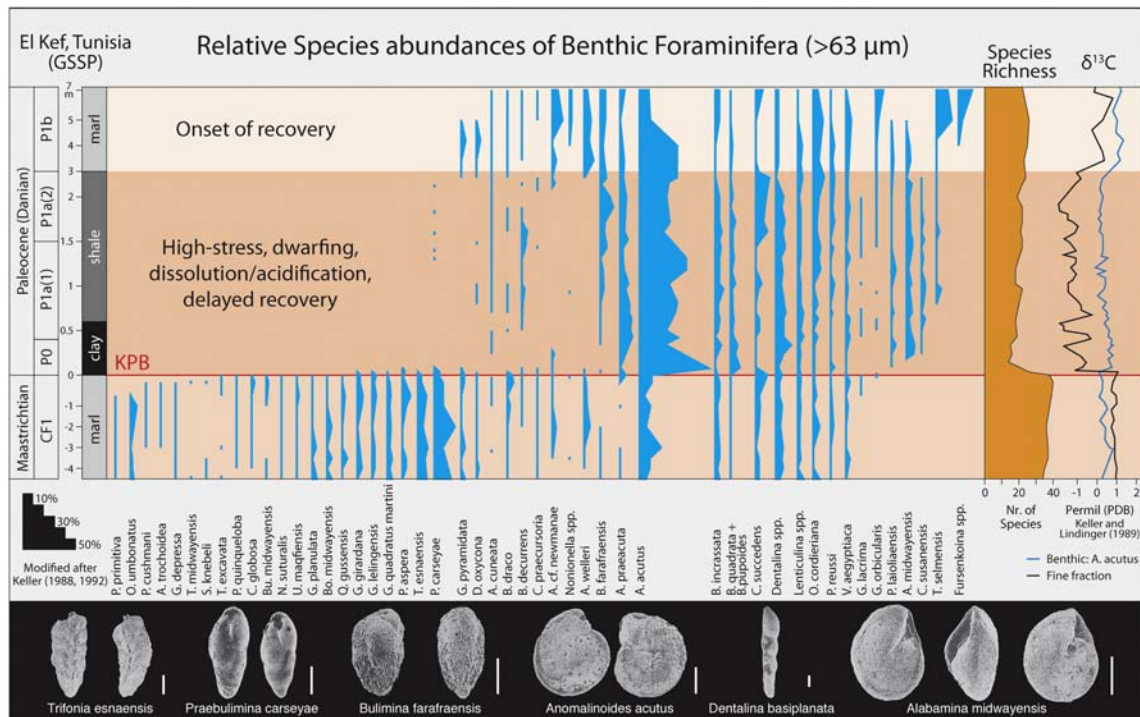
Fig. 9. Relative abundances of benthic foraminifera (>63 \mu\text{m} ) and carbon stable isotopes of bulk rock and benthic species Anomalinoidea acutus across the KPb transition at El Kef, Tunisia. Note the major faunal turnover across the KPb with up to 48% species disappearing over 500 ky with many of them reappearing after environmental recovery. Faunal data from Keller (1988b); stable isotope data from Keller and Lindinger (1989).
