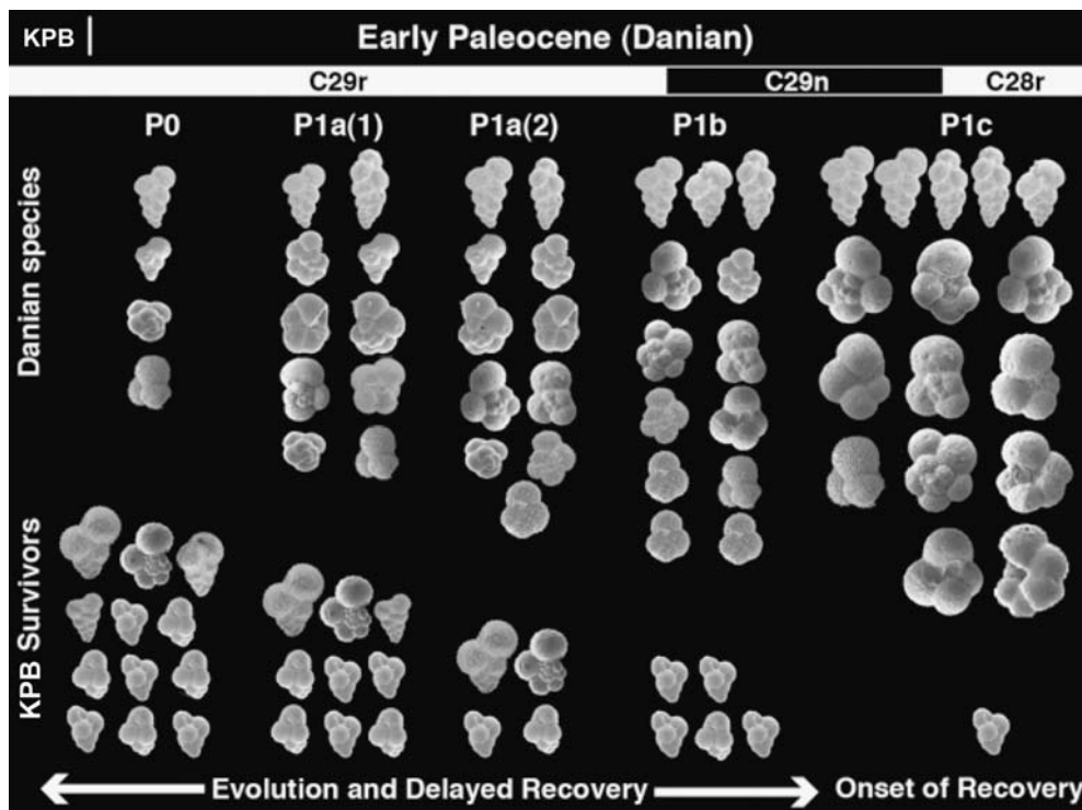
Fig. 8. Early Danian evolution and decline in Cretaceous survivor species illustrate high-stress environments. Small dwarfed species and low diversity mark delayed marine recovery in magnetochron C29r from zones P0 through P1a(2) correlative with decreasing abundance and gradual extinction of dwarfed survivor species. The last phase of Deccan volcanism began near the zone P1a/P1b boundary (C29r/C29n) and marks the extinction of two dominant zone P1a index species ( Parvularugoglobigerina eugubina , P. longiapertura ). Marine recovery begins after this last volcanic phase and is marked by higher diversity and increasing species sizes. Note the number of the same specimens in each column indicates relative abundance. From Puneekar et al. (2014).
