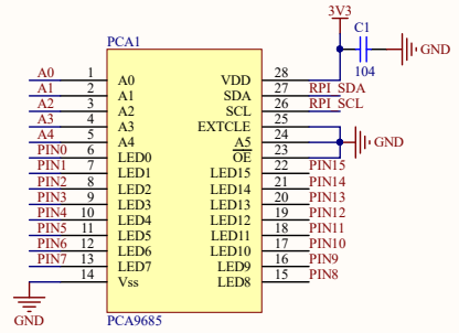
I2C to PWM
