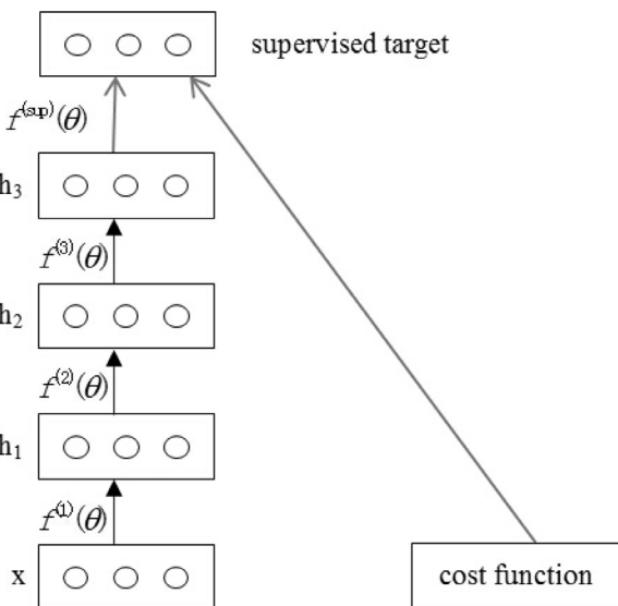
Fig. 4. Stacked auto-encoder for fine-tuning.
