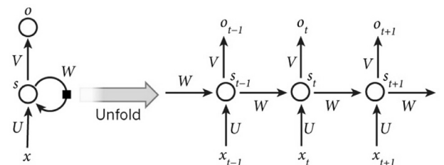
Fig. 8. Recurrent neural network.
