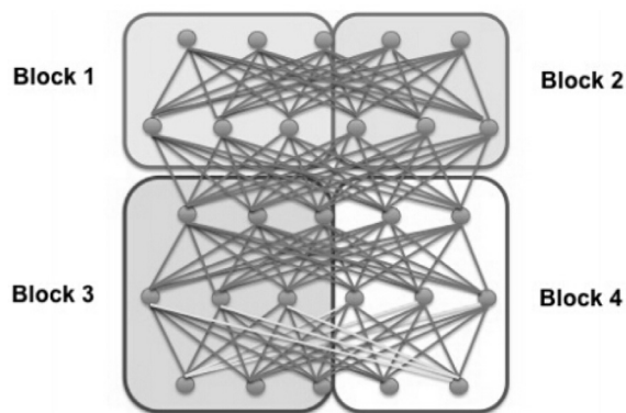
Fig. 10. Example of DistBelief with four blocks.
