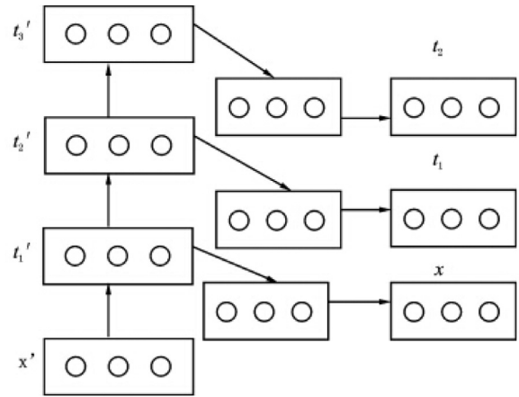
Fig. 17. Deep imputation network.
