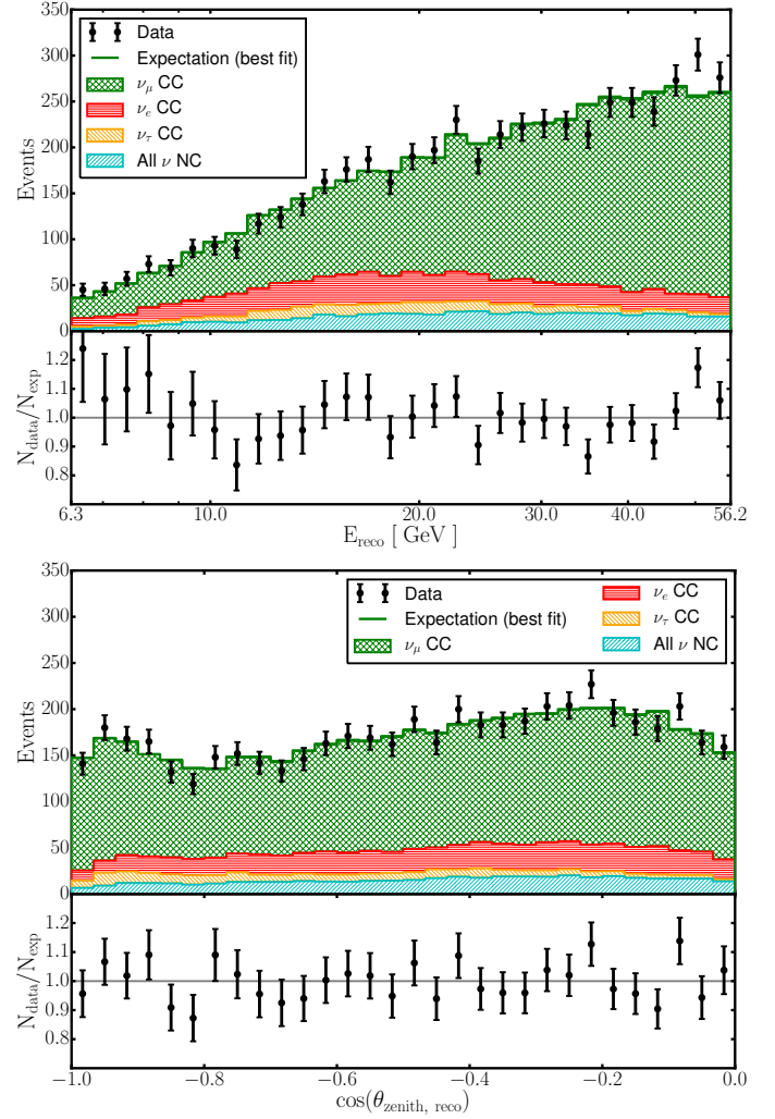
FIG. 8. Event rates shown as a function of (top) E_{\text{reco}} and (bottom) \cos\theta_{z, \text{reco}} . The various different neutrino components from Monte Carlo simulation used in the fit are shown as stacked histograms. The total expected event rate is in good agreement with the observed data, shown as black points.
