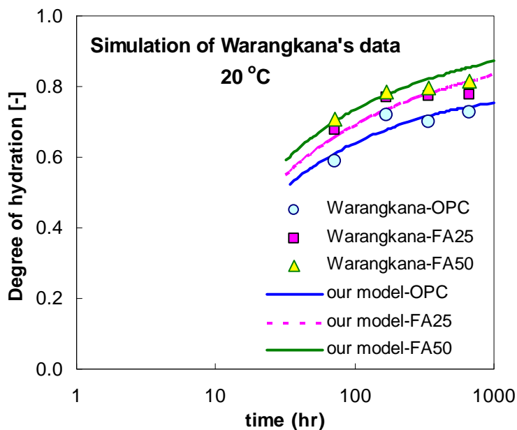
Figure 10 Simulation of the progress of the degree of cement hydration in Warangkana's work [12]
