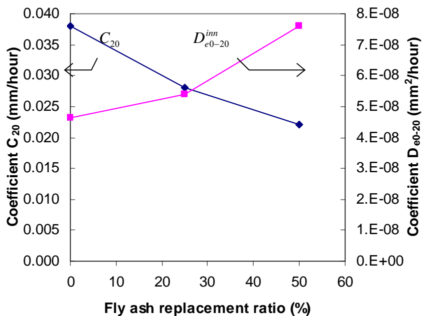
Figure 7 Effect of the fly ash replacement ratio on the reaction coefficient C_{20} (left, blue) and the effective diffusion coefficient D_{e0-20}^{inn} (right, purple)
