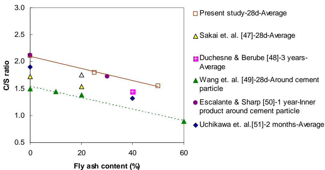
Figure 8 Effect of the fly ash replacement ratio on the Ca/Si molar ratio of C-S-H gel
