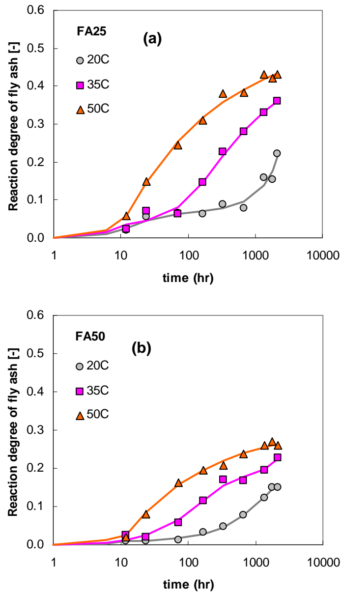
Figure 6 Progress of the degree of pozzolanic reaction of fly ash at three (20 °C, 35 °C, and 50 °C) curing temperatures: (a) FA25 paste, (b) FA50 paste
