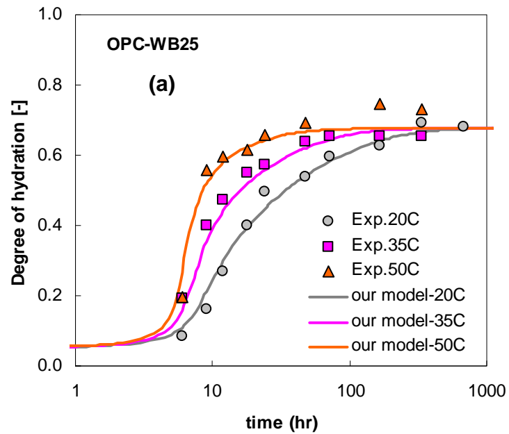
Figure 5 Simulation of the progress of the degree of cement hydration of fly ash-cement paste with w/b = 0.25 : (a) OPC paste, (b) FA25 paste, (c) FA50 paste, (d) different fly ash-cement pastes at 20 °C
