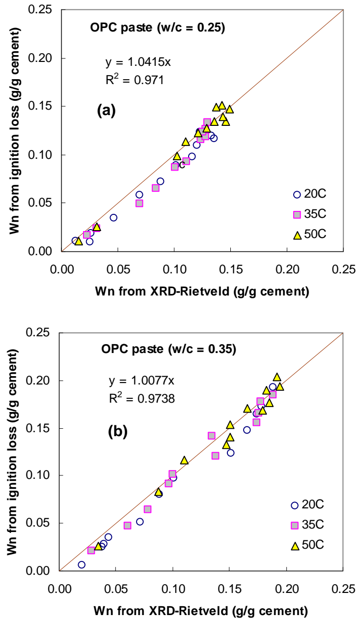
Figure 2 Correlation between non-evaporable water calculated from the degree of hydration and non-evaporable water measured from the ignition loss; (a) w/b = 0.25 and (b) w/b = 0.35
