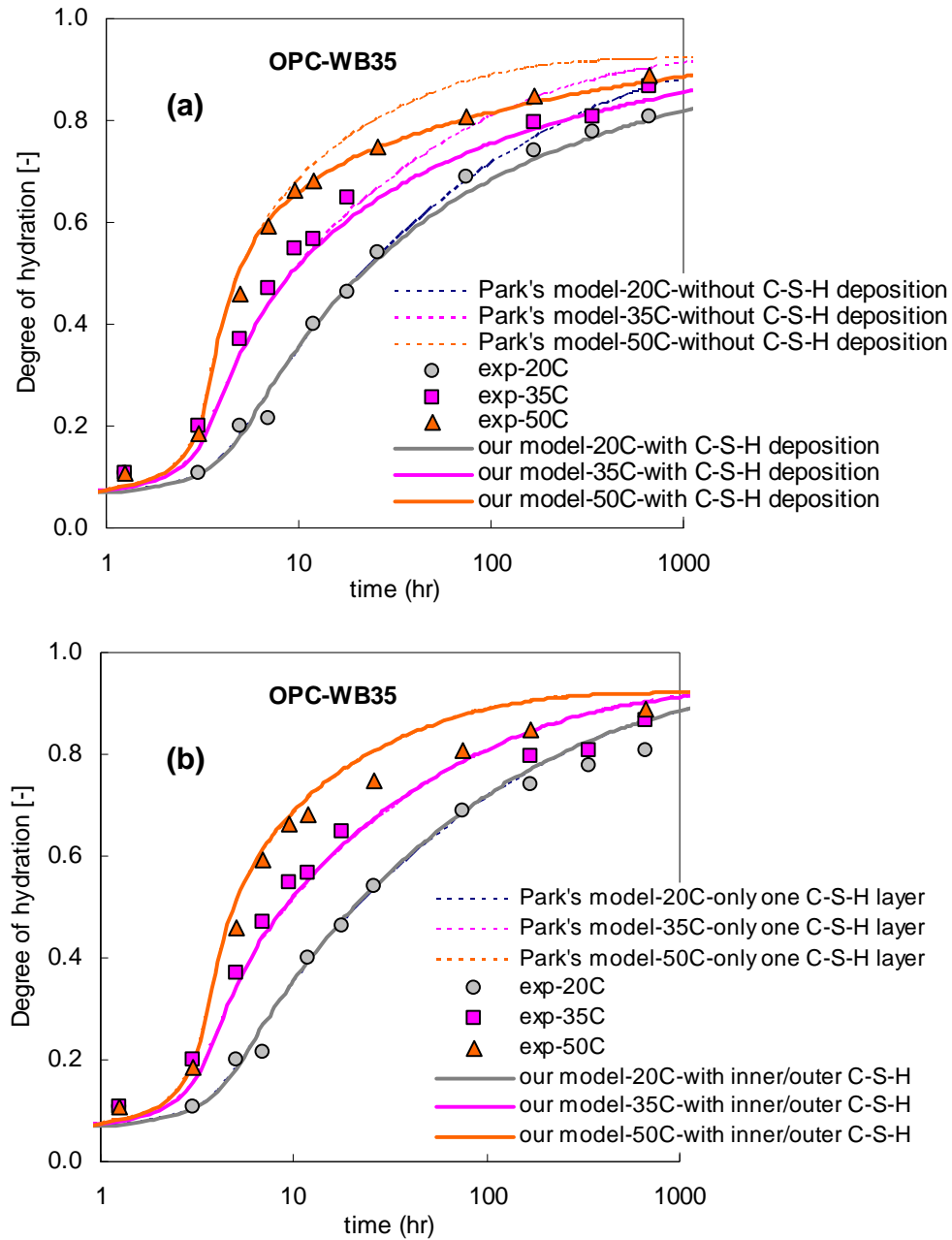
Figure 4 Simulation of the progress of the degree of cement hydration of Portland cement paste with w/b = 0.35 , (a) effect of C-S-H particle deposition, (b) effect of differences in effective diffusion coefficient of the inner and the outer C-S-H gel
