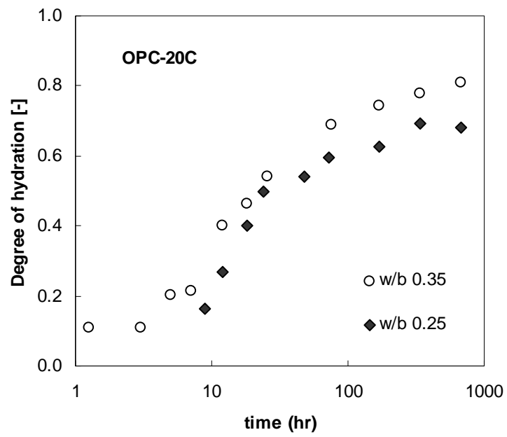
Figure 3 Degree of hydration of OPC pastes cured at 20 °C
