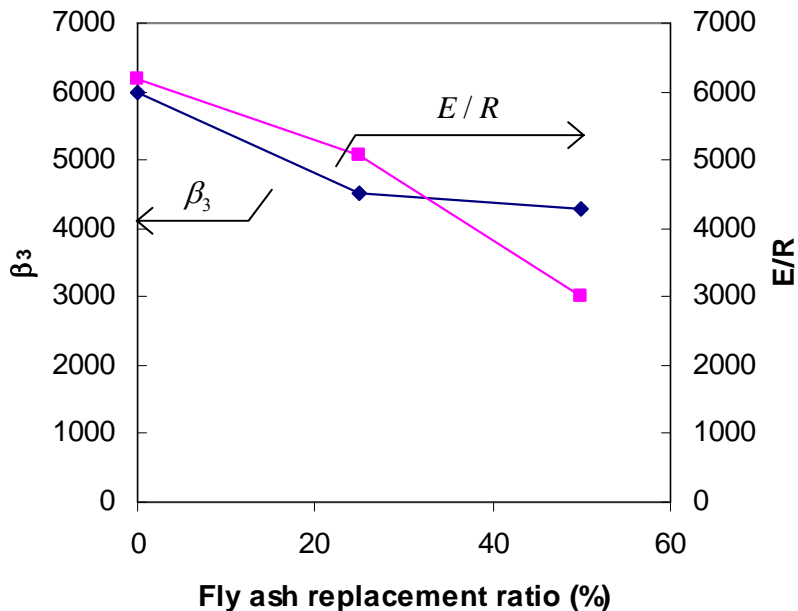
Figure 9 Effect of the fly ash replacement ratio on the temperature sensitivity of the diffusion process \beta_3 (left, blue) and of the chemical reaction E/R (right, purple)
